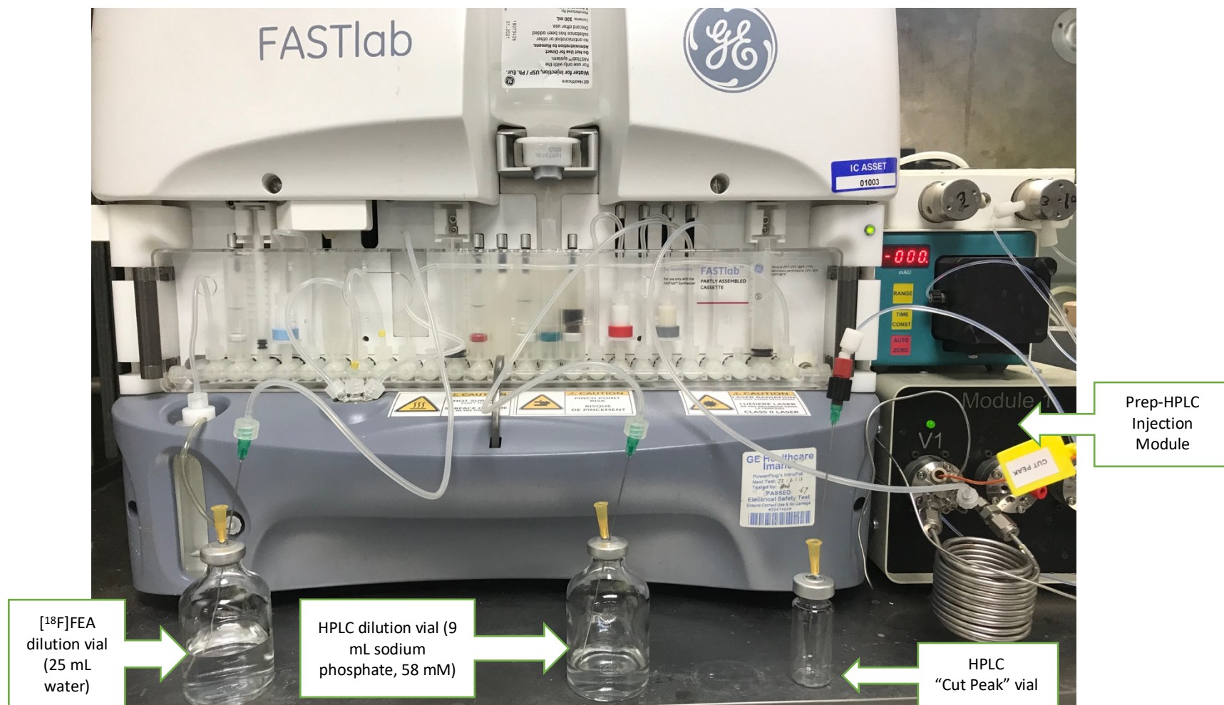
Figure 1. Photograph of FASTlab™ setup.
