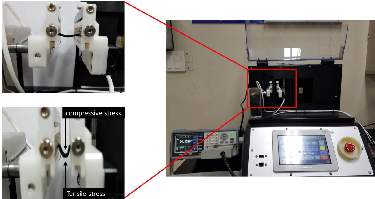
Figure S2. Images of the multi-purpose flexible test machine
