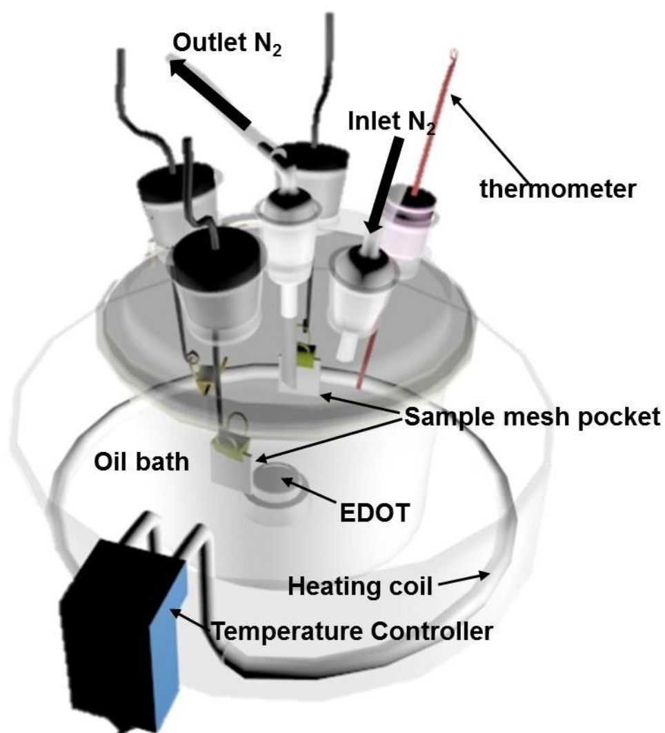
Figure S1. Schematic diagram of VPP chamber
