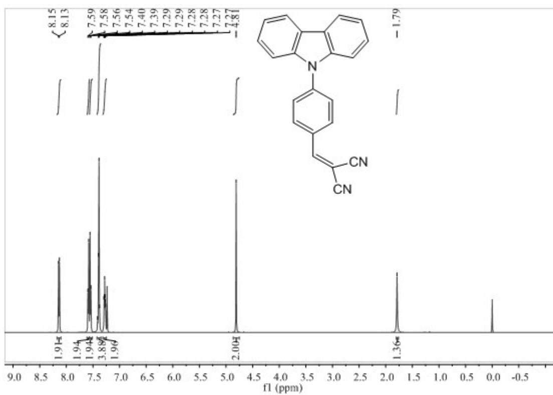
Fig. S1 ^1\text{H} NMR of CBM.
