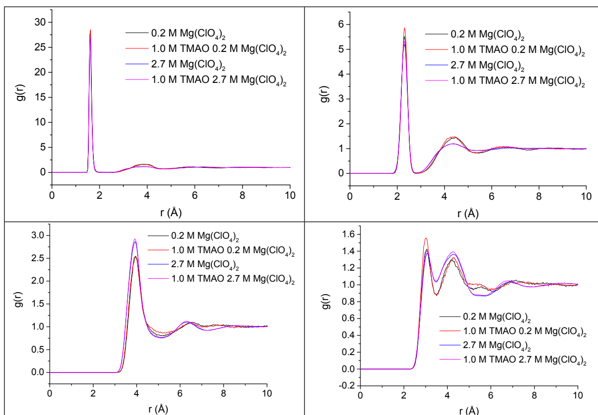
Figure S6. \text{MgO}_w site-site RDFs (top left), \text{MgH}_w site-site RDFs (top right), \text{Cl}_p\text{O}_w site-site RDFs (bottom left), \text{Cl}_p\text{H}_w site-site RDFs (bottom right)
