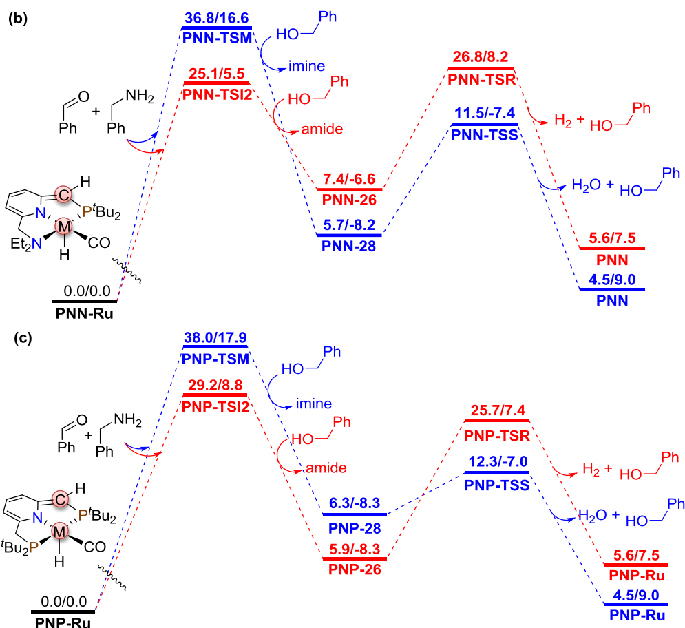
Fig. S5. The dehydrogenation or dehydration of hemiaminal heam via (a) non-catalyzed, (b) PNN-Ru catalyzed, and (c) PNP-Ru catalyzed reactions.
