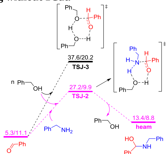
Fig. S2. Free energy profiles for amine and alcohol coupling ( Route g ) or alcohol and alcohol coupling without 1Cat . Free energy/enthalpy values are in kcal/mol.
