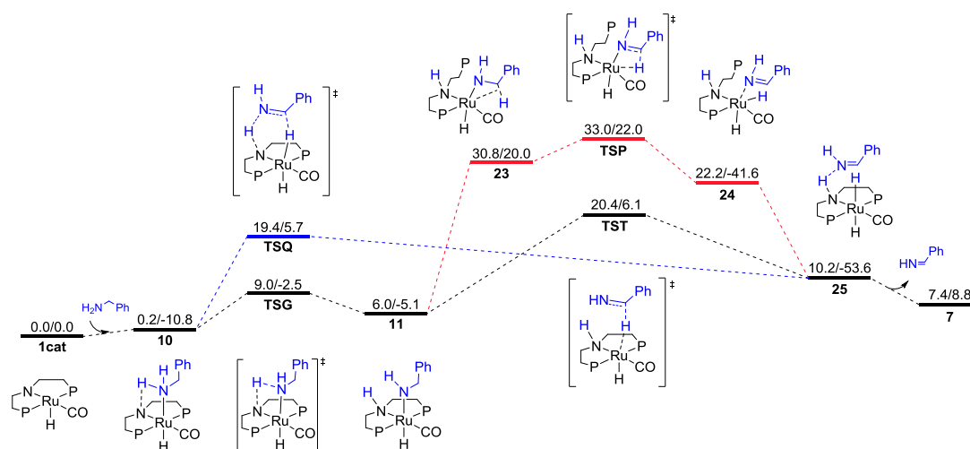
Fig. S1. Free energy profiles for the Macho-Ru catalyzed dehydrogenation of amine. Free energy/enthalpy values are in kcal/mol.
