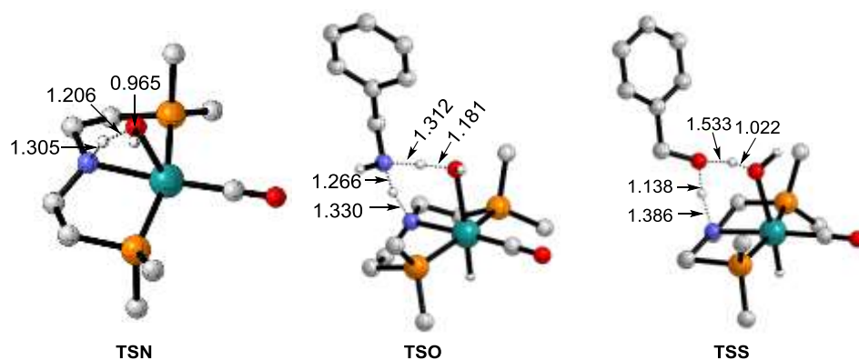
Fig. S4. Optimized transition state structures for elimination of water from complex 20 , along with the key bond lengths (in Å). Trivial hydrogen atoms are omitted for clarity.
