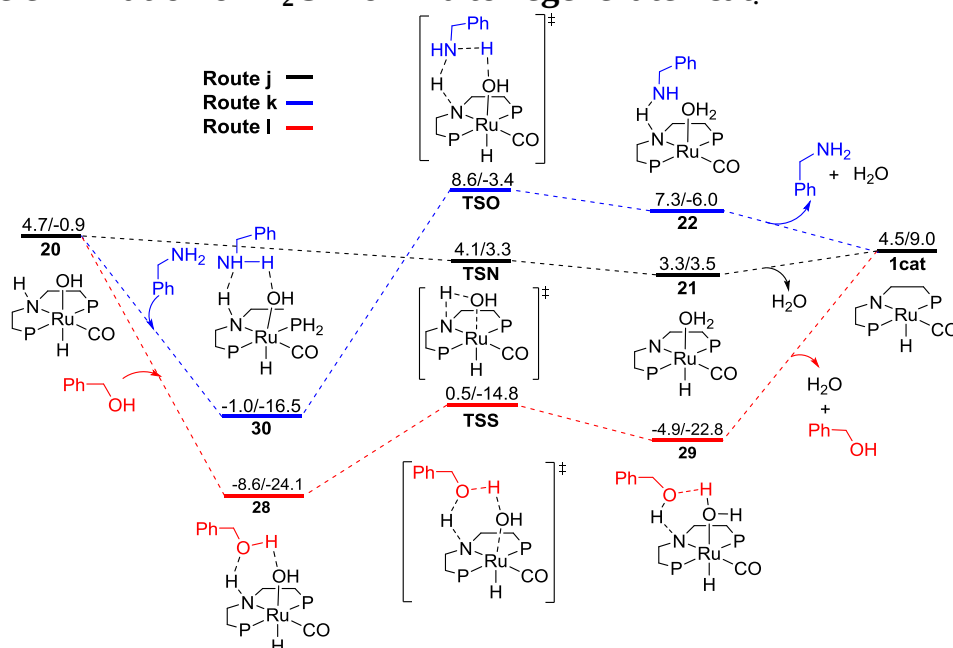
Fig. S3. Free Energy profiles of possible reaction pathways for the elimination of H 2 O from 20 .
