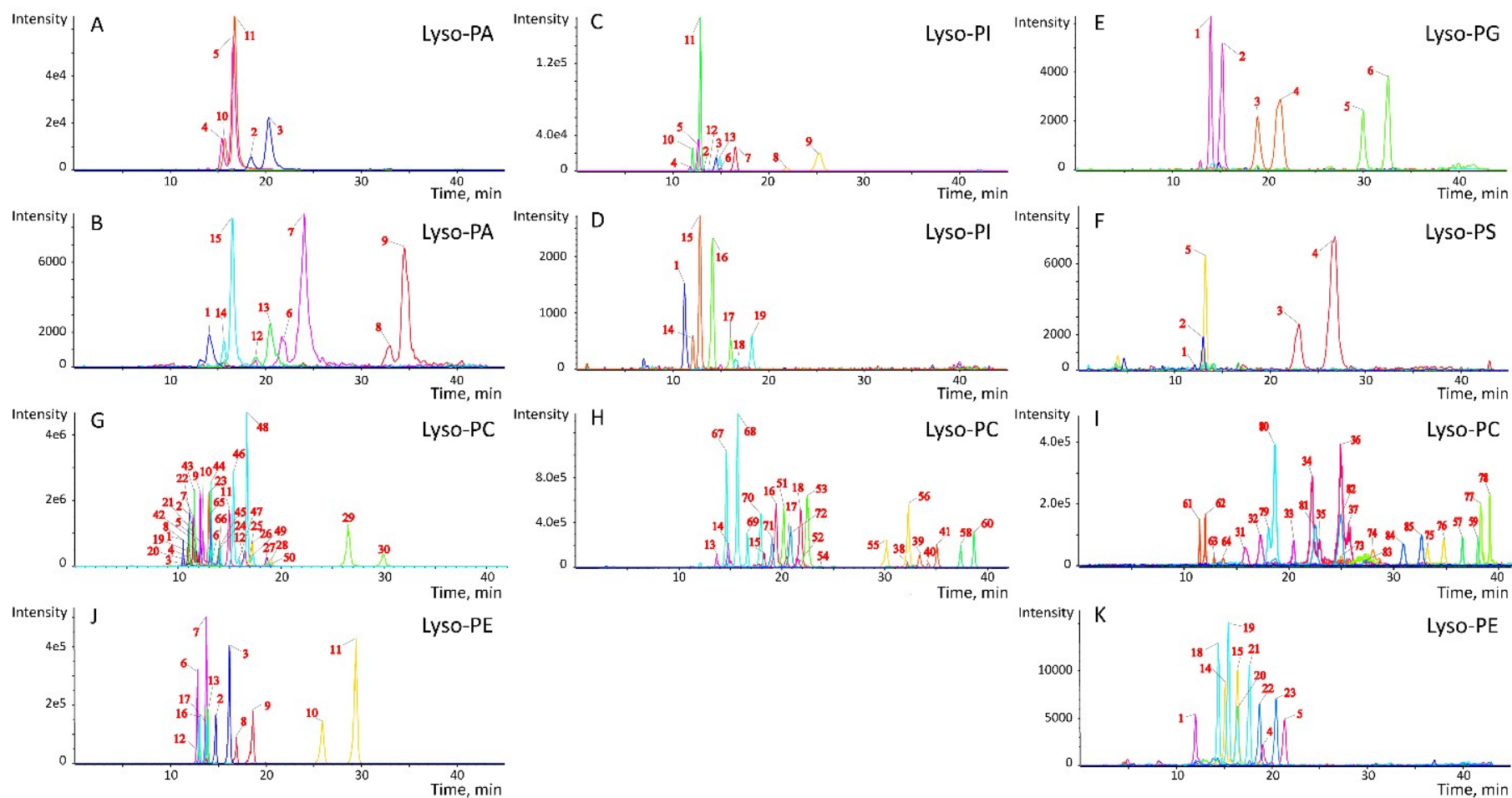
Figure S1. The established metabolite profile of endogenous Lyso-GPL. The extracted ion chromatograms were extracted individually according to the different peak intensities to clearly display all of the peaks from the LC-QTRAP-MRM analysis.
