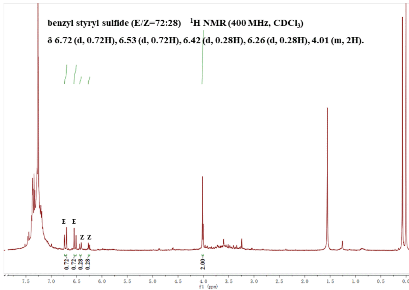
Fig. S1 NMR spectra of benzyl styryl sulfide.
