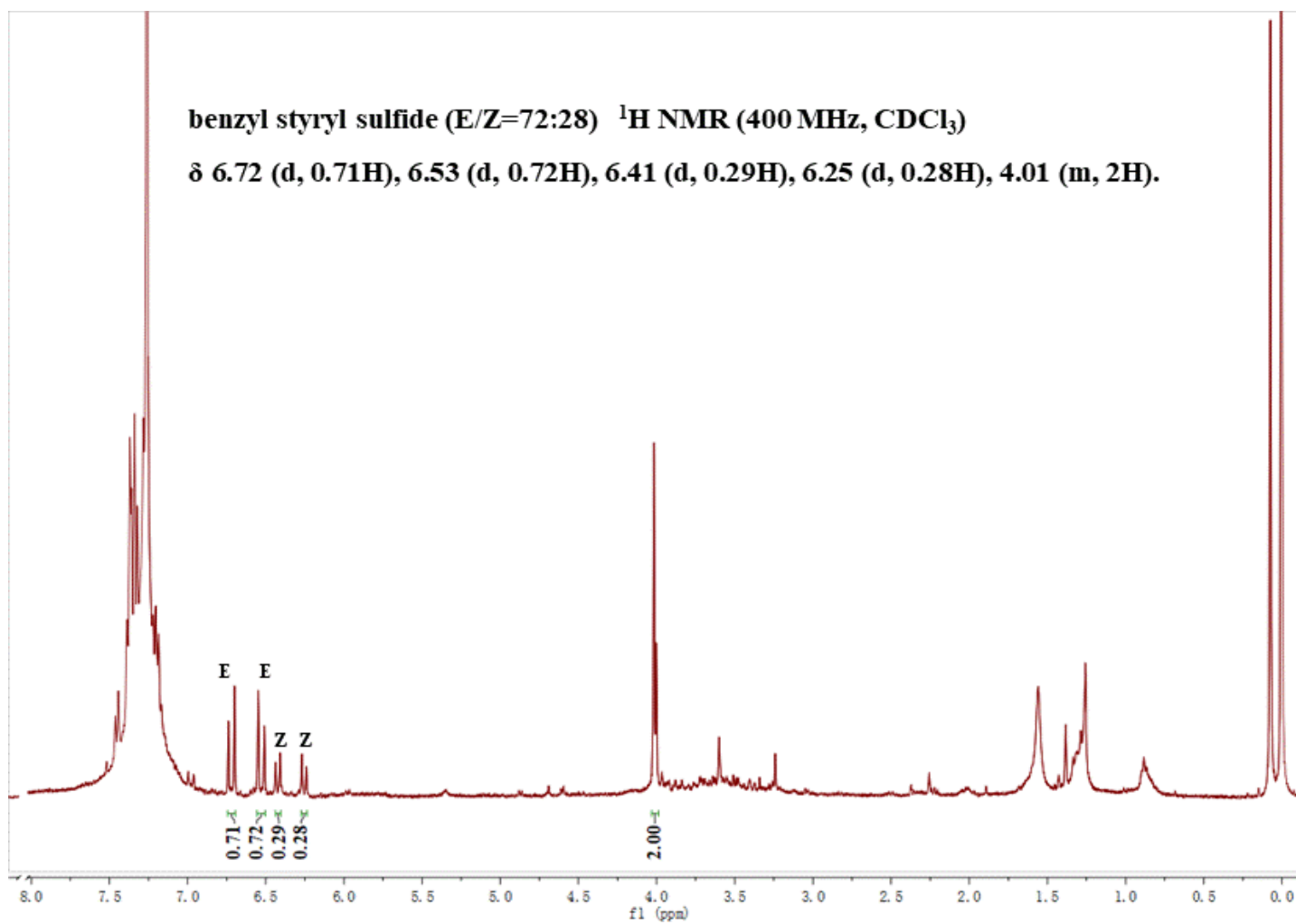
Fig. S2 NMR spectra of benzyl styryl sulfide after irradiated for another 15h.
