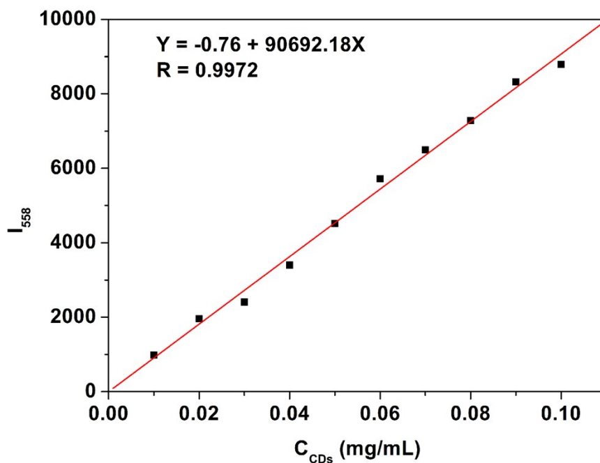
Fig. S8 The linearity of emission intensity at 558 nm to increasing CDs concentration.
