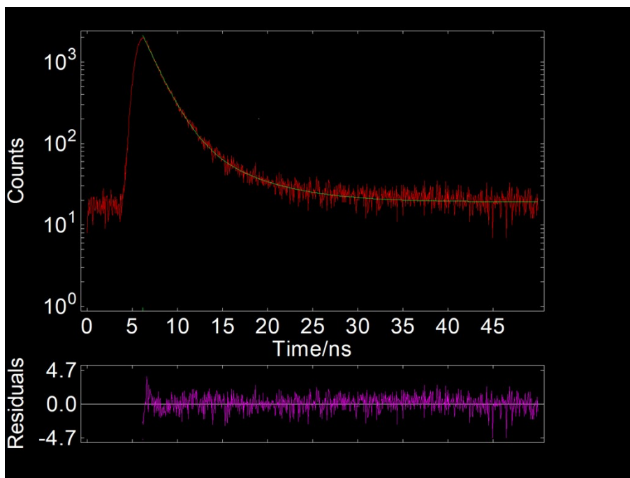
Fig. S4 Lifetime curve of CDs (0.02 mg/mL in 100% water, emission wavelength was 430 nm) with excitation at 376 nm.
