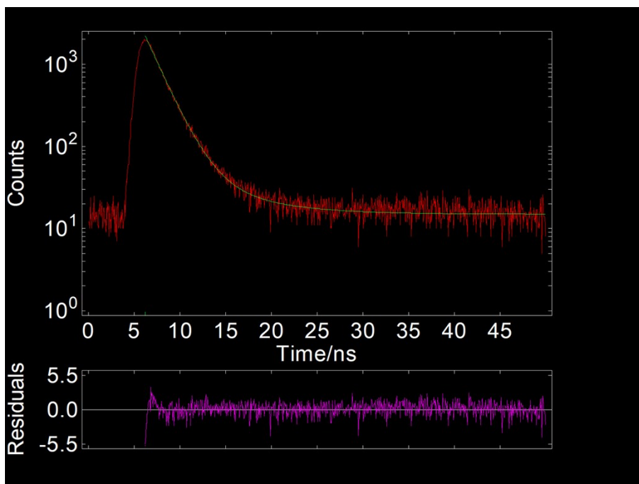
Fig. S7 After addition of Arg ( 1.0 \times 10^{-4} M in water), the lifetime curve of CDs (0.02 mg/mL in 100% water, emission wavelength was 570 nm) with excitation at 376 nm.
