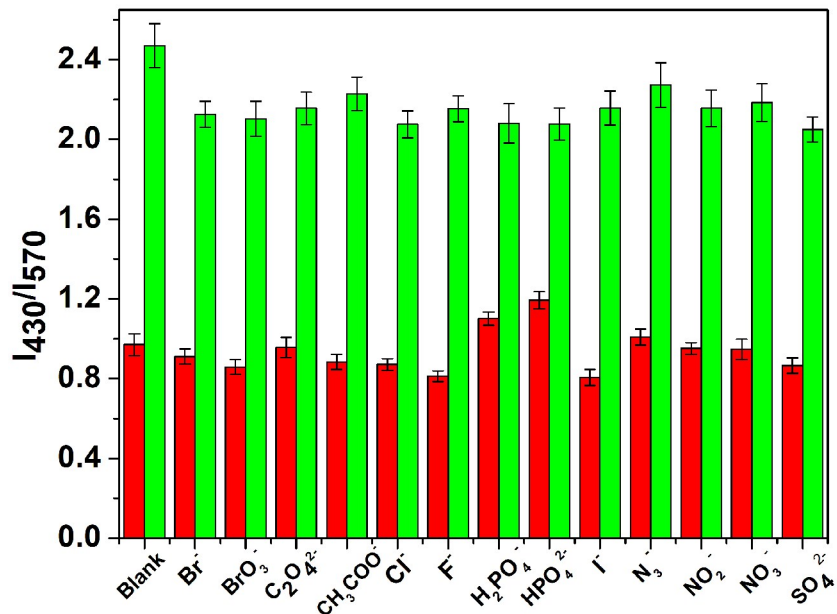
Fig. S3 Fluorescence responses of CDs (0.02 mg/mL in 100% water) upon addition of different anions ( 1.0 \times 10^{-4} M) (red bars), and fluorescence changes of the mixture of CDs (0.02 mg/mL in 100% water) and Arg ( 1.0 \times 10^{-4} M in water) after addition of the indicated anions ( 1.0 \times 10^{-4} M) (green bars). The excitation was at 376 nm. I_{430} and I_{570} represent the fluorescence intensity at 430 nm and 570 nm.
