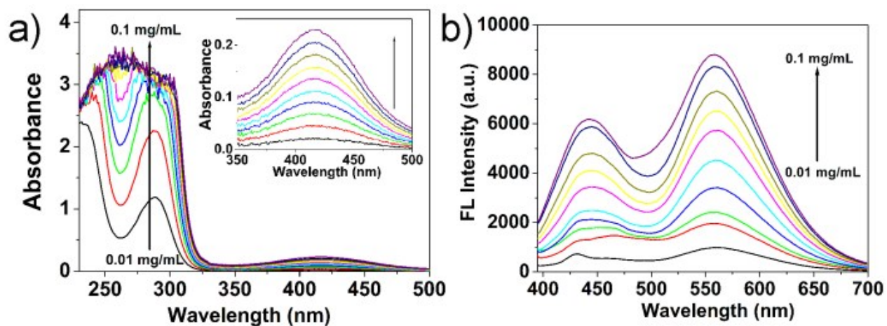
Fig. S1 (a) Absorption spectra of CDs water solution in different concentration conditions. Insert of (a) Amplified absorption spectra of CDs from 350 to 500 nm. (b) Emission spectra of CDs water solution in different concentration conditions with excitation at 376 nm.
