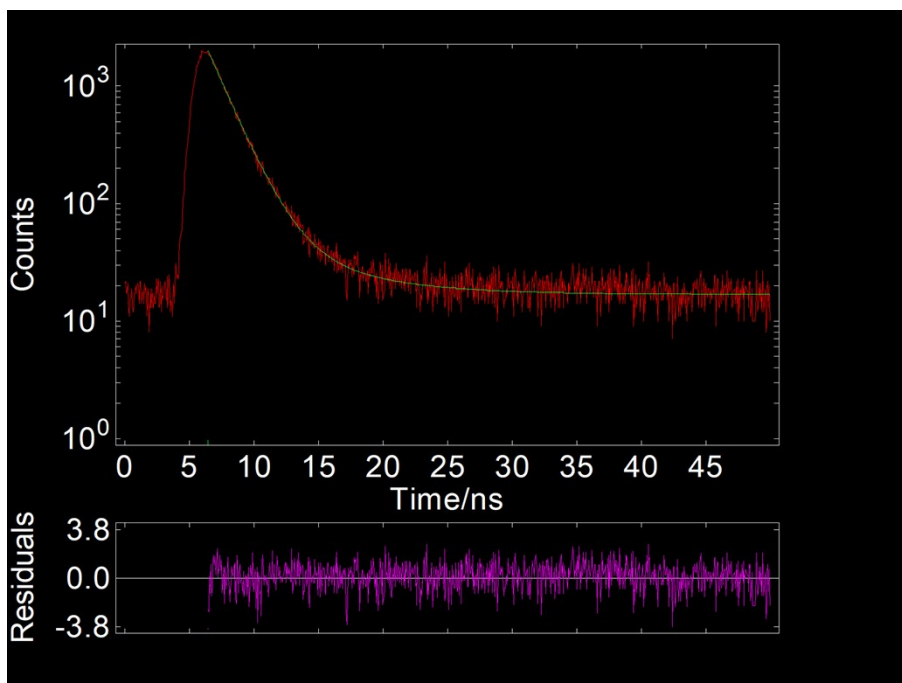
Fig. S5 Lifetime curve of CDs (0.02 mg/mL in 100% water, emission wavelength was 570 nm) with excitation at 376 nm.
