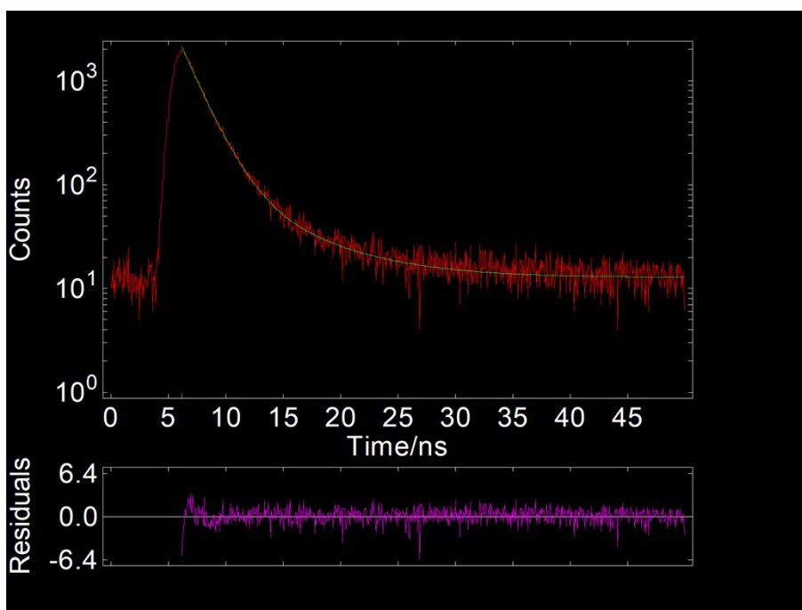
Fig. S6 After addition of Arg ( 1.0 \times 10^{-4} M in water), the lifetime curve of CDs (0.02 mg/mL in 100% water, emission wavelength was 430 nm) with excitation at 376 nm.
