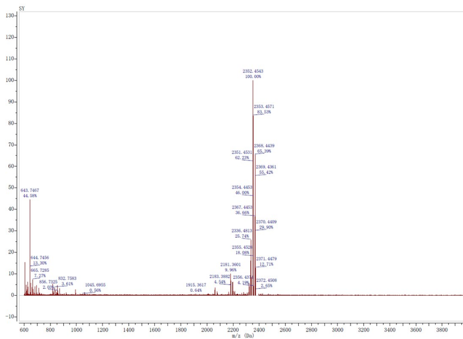
Fig. S1. Section of MALDI-TOF mass spectrum of C4A-NO 2 .
