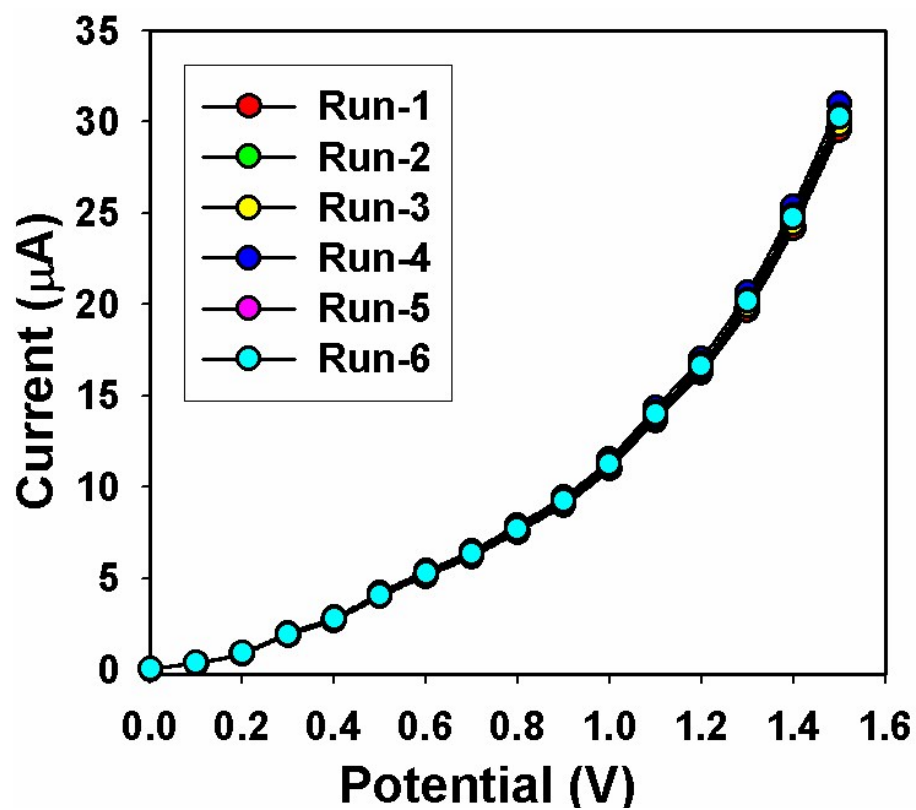
Fig. S2: Stability of the Ag/ZnO/Nafion/GCE fabricated sensor was studied for detection of melamine with different time interval (30 mins) from Run-1 to Run-6 in identical conditions.
