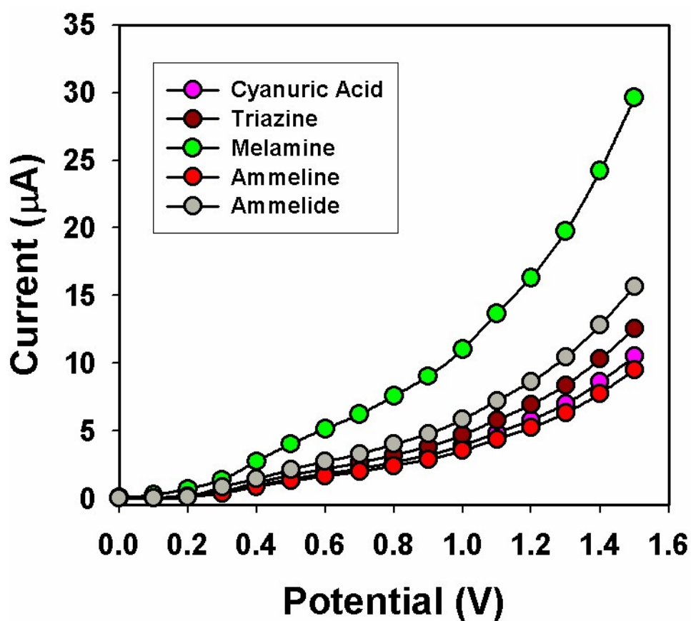
Fig. S1: Electrochemical response with similar compound by using Ag/ZnO/Nafion/GCE sensor materials in identical conditions.
