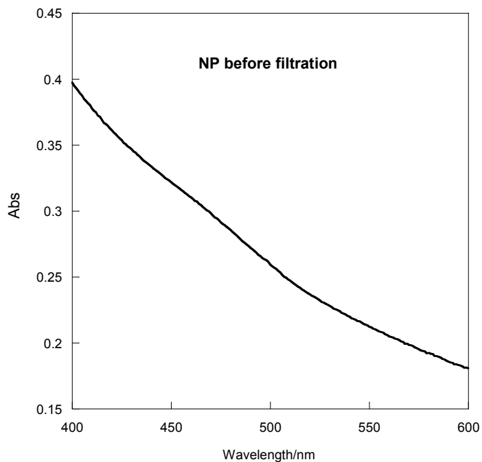
Figure S1. Absorption of the n- \pi transition band of the DK4/PBCA nanoparticle before (up) and after filtration (down).
