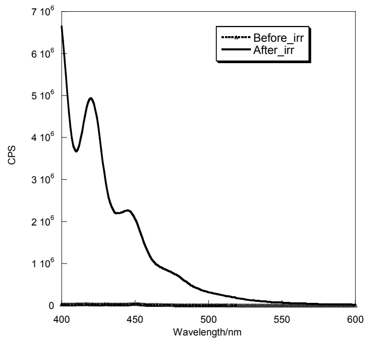
Figure S2. Fluorescence spectra of DK4/PBCA nanoparticle (after filtration) before and after irradiation (excitation wavelength 390 nm).
