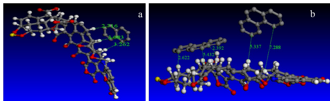
Fig. S3 Optimized geometrical structures and the adsorption processes of NAP (a) and PHE (b) on WAC.
