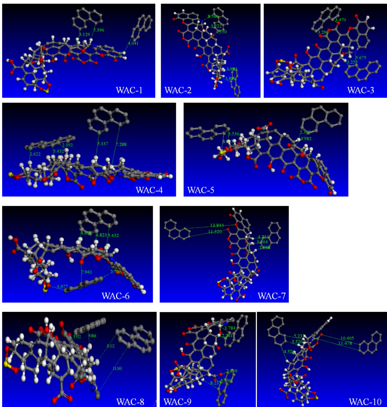
Fig. S2 Optimized geometrical structures and the adsorption processes of PHE on WAC
