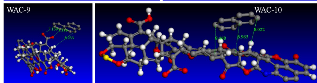
Fig. S1 Optimized geometrical structures and the adsorption processes of NAP on WAC.
