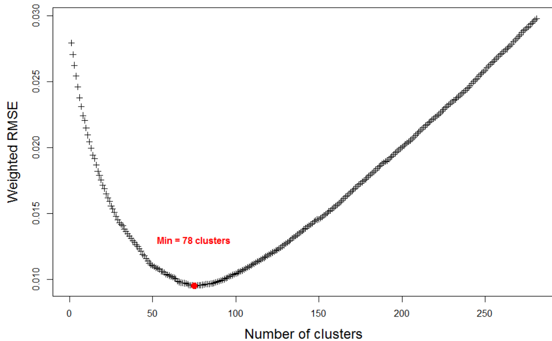
L-method for silhouette graph
