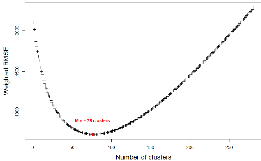
L-method for elbow graph
