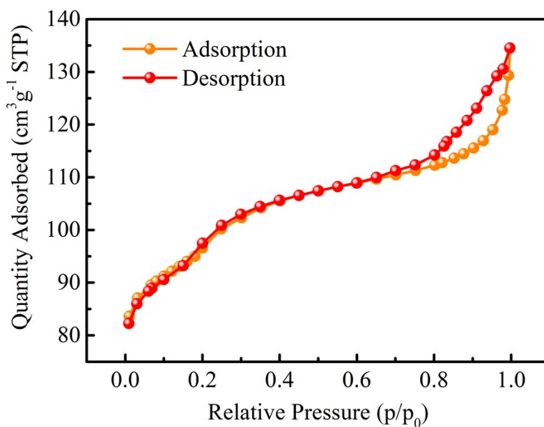
Fig. S1. Isotherm linear plots of Brunauer-Emmett-Teller (BET) surface area test of V_4Nb_{18}O_{55} nanofibers.
