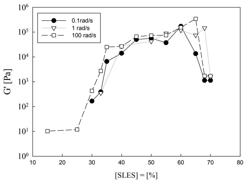
Figure 2s. Elastic modulus evaluated at 0.1-1-100 rad/s as function of the SLES concentration.
