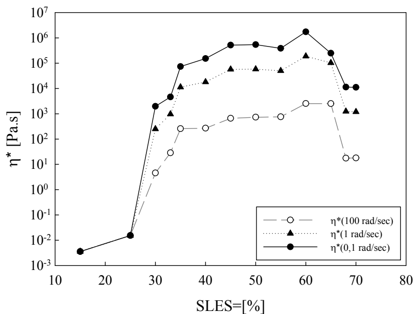
Figure 1s. Complex viscosity evaluated at 0.1-1-100 rad/s as function of the SLES concentration.
