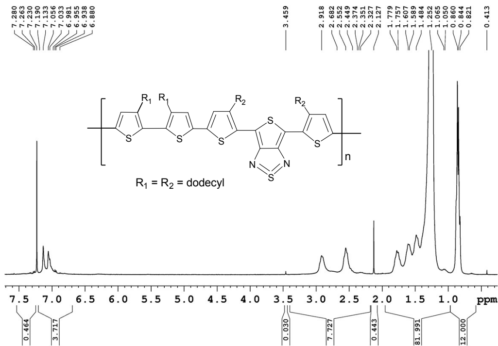
Figure S5: ^1\text{H NMR} spectrum of poly[4,6-bis(3'-dodecylthiophen-2'-yl)thieno[3,4-c][1,2,5]thiadiazole-5',5'-diyl-alt-3,3'-didodecyl-2,2'-bithiophene-5,5'-diyl] ( CDTDBT ) in \text{CDCl}_3 .
