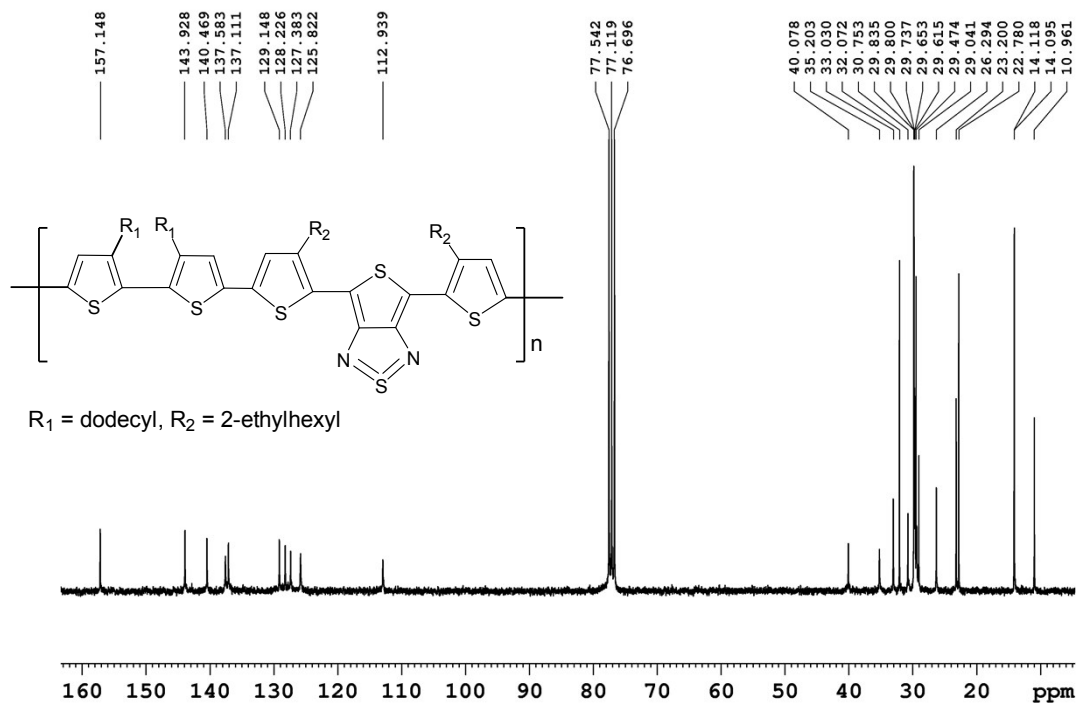
Figure S8: ^{13}\text{C NMR} spectrum of poly[4,6-bis(3'-(2-ethylhexyl)thiophen-2'-yl)thieno[3,4-c][1,2,5]thiadiazole-5',5'-diyl- alt -3,3'-didodecyl-2,2'-bithiophene-5,5'-diyl] (CEHTDBT) in \text{CDCl}_3 .
