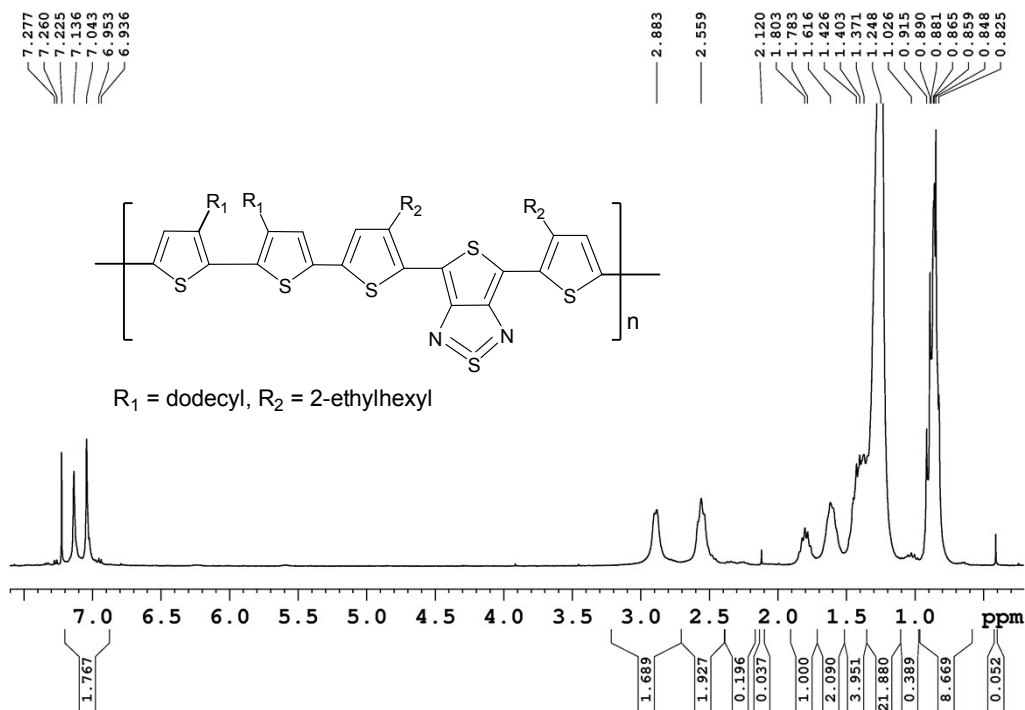
Figure S7: ^1\text{H NMR} spectrum of poly[4,6-bis(3'-(2-ethylhexyl)thiophen-2'-yl)thieno[3,4-c][1,2,5]thiadiazole-5',5'-diyl- alt -3,3'-didodecyl-2,2'-bithiophene-5,5'-diyl] (CEHTDBT) in \text{CDCl}_3 .
