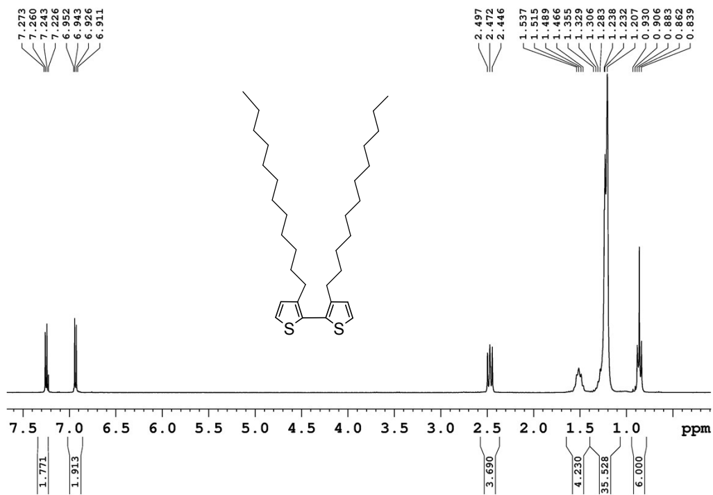
Figure S1: ^1\text{H} NMR spectrum of 3,3'-didodecyl-2,2'-bithiophene ( 1 ) in \text{CDCl}_3 .
