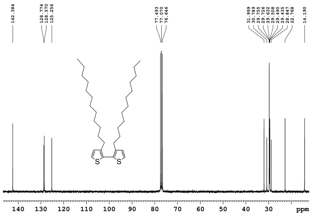
Figure S2: ^{13}\text{C} NMR spectrum of 3,3'-didodecyl-2,2'-bithiophene ( 1 ) in \text{CDCl}_3 .
