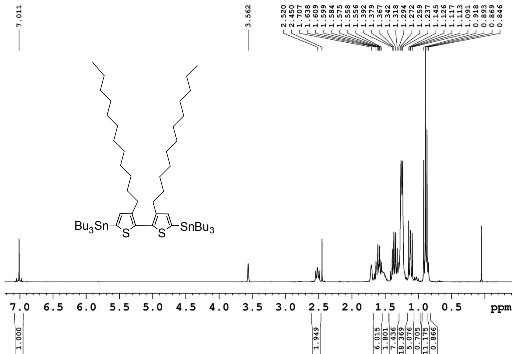
Figure S3: 1 H NMR spectrum of 3,3'-didodecyl-5,5'-tributylstannyl-2,2'-bithiophene ( 2 ) in deuterated tetrahydrofuran.
