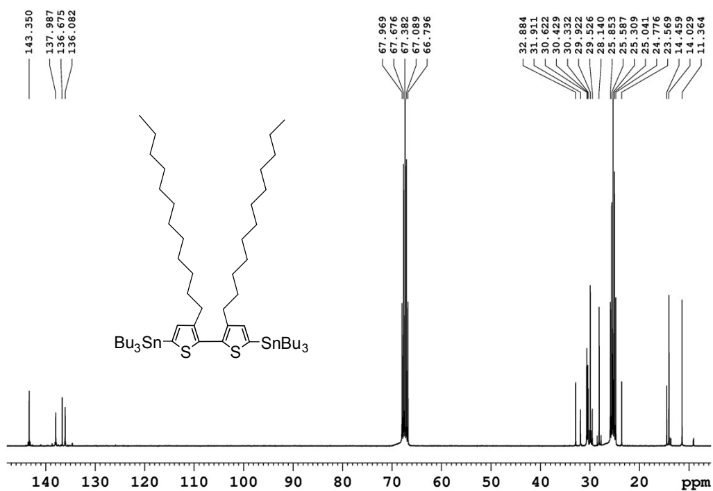
Figure S4: 13 C NMR spectrum of 3,3'-didodecyl-5,5'-tributylstannyl-2,2'-bithiophene ( 2 ) in deuterated tetrahydrofuran.
