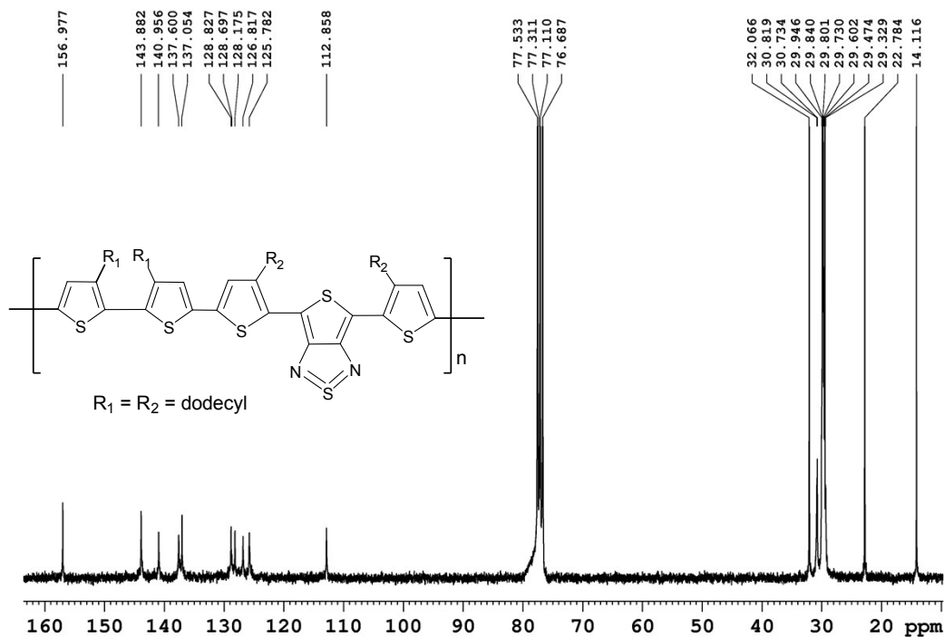
Figure S6: ^{13}\text{C NMR} spectrum of poly[4,6-bis(3'-dodecylthiophen-2'-yl)thieno[3,4-c][1,2,5]thiadiazole-5',5'-diyl-alt-3,3'-didodecyl-2,2'-bithiophene-5,5'-diyl] ( CDTDBT ) in \text{CDCl}_3 .
