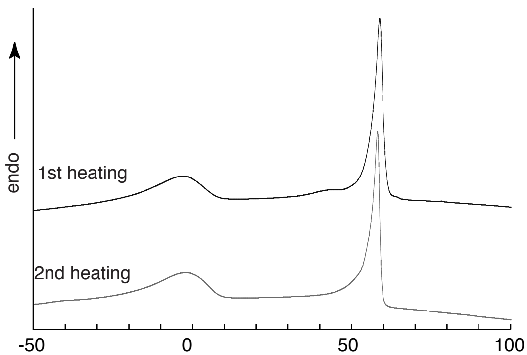
Fig. DSC curves of the fiber sample (temperature scan rate 20°C min -1 ).
