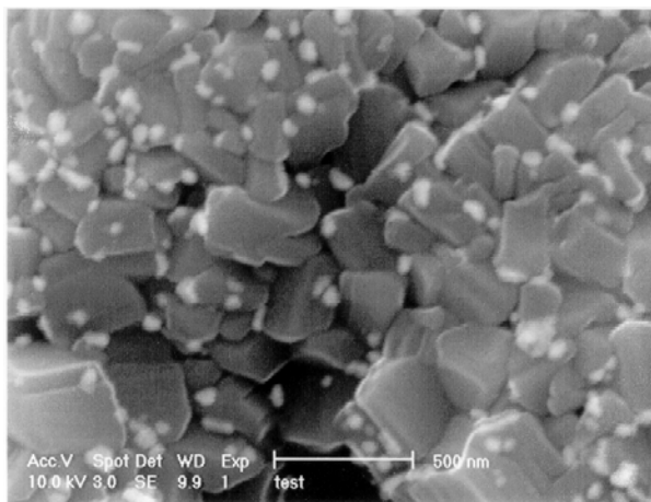
c) SEM of Pd(0)-mordenite (4 wt.% Pd), autoreduced by N 2 .
