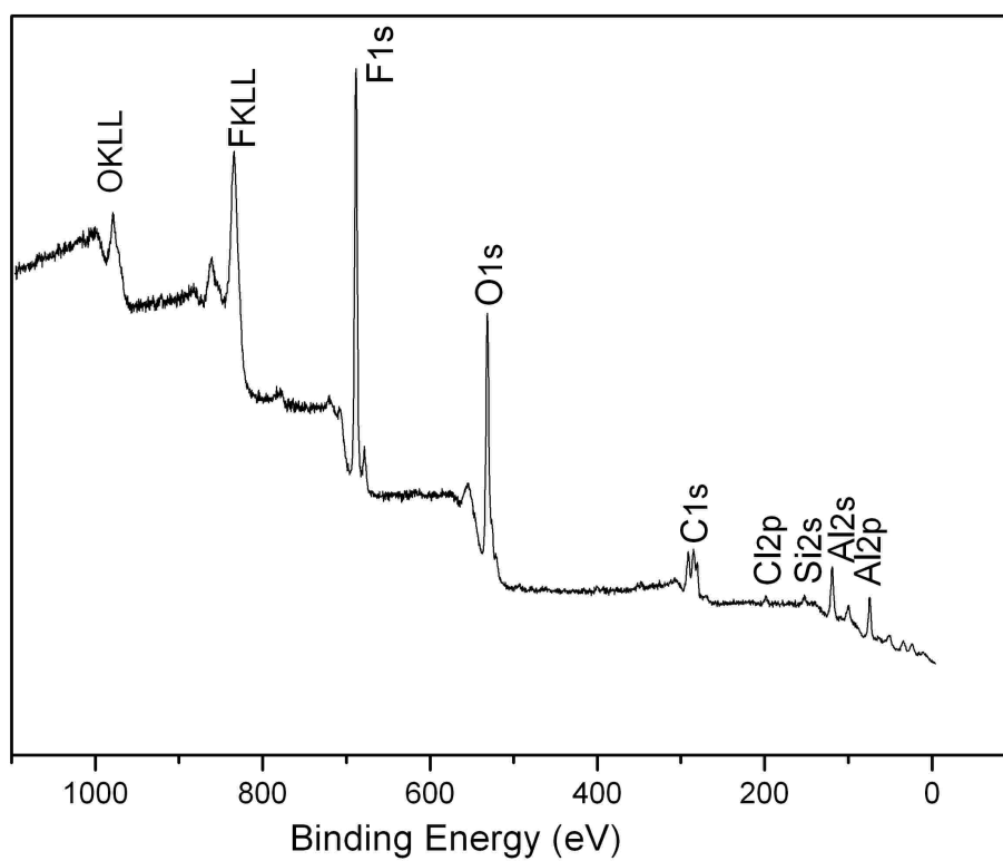
Figure S1. Full XPS survey of perfluorinated alumina.
