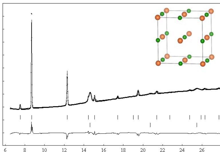
Figure S1. Preliminary Rietveld analysis plot excluding H atoms.
