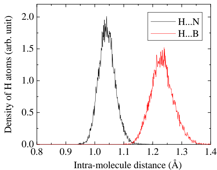
Figure S2. The distribution of H atoms with respect to the distance to the nearest B atoms (red) and N atoms (black), from ab initio MD calculations.
