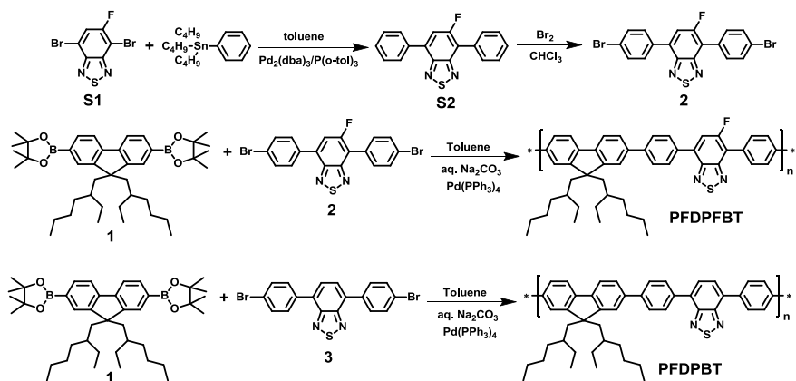
Scheme S1. The synthetic route of monomers and polymers.
