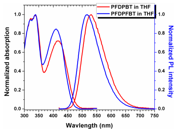
Fig. S4. The UV-Vis absorption and fluorescence spectra of PFDPBT and PFDPFBT in THF solution.
