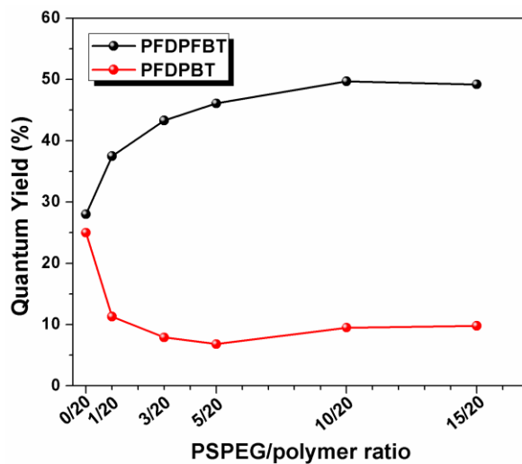
Fig. S1. The quantum yield changes of different PS-PEG-COOH concentration at 20 ppm polymer.
