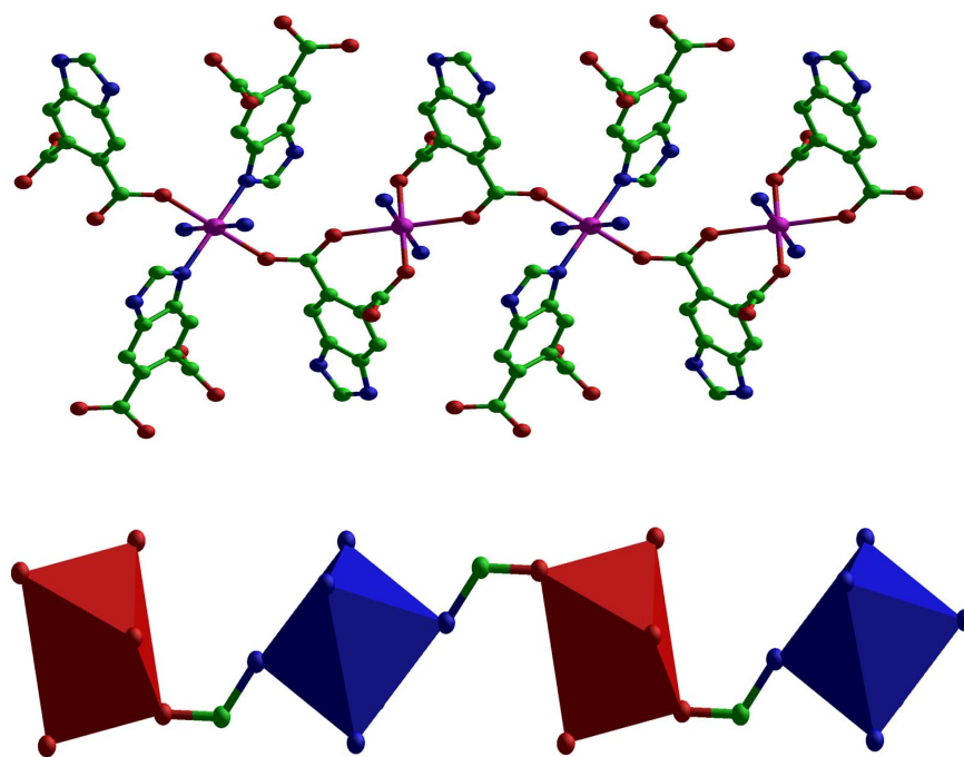
Figure S3. View of the 1D [Co(Hbidc)] n zigzag chain in 1 .
