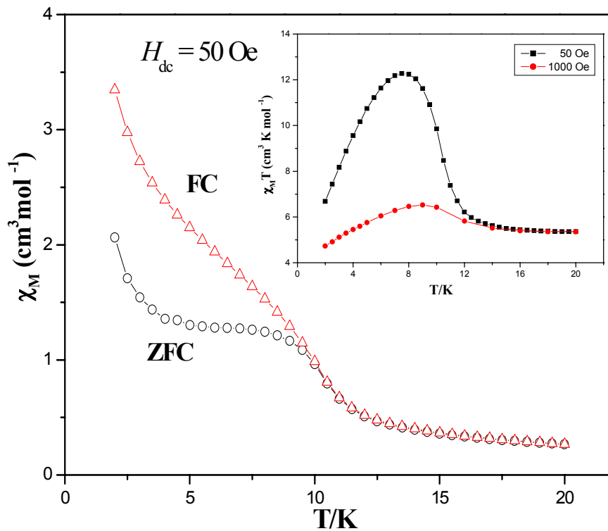
Figure S4. Field-cooled (FC) and zero-field-cooled (ZFC) magnetization for 1. The inset is the plots of \chi_M T vs. T at various fields.
