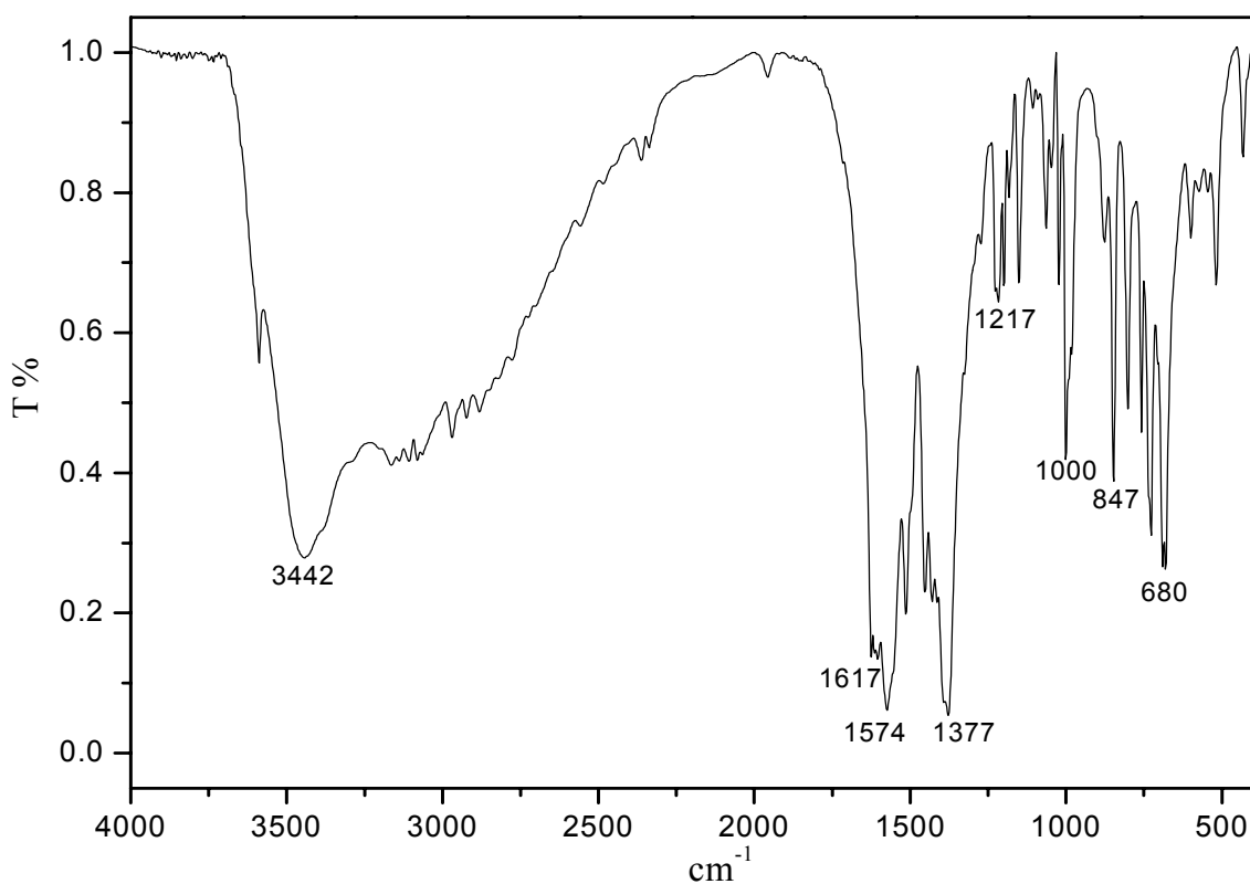
Figure S1. The IR spectra of complex 1
