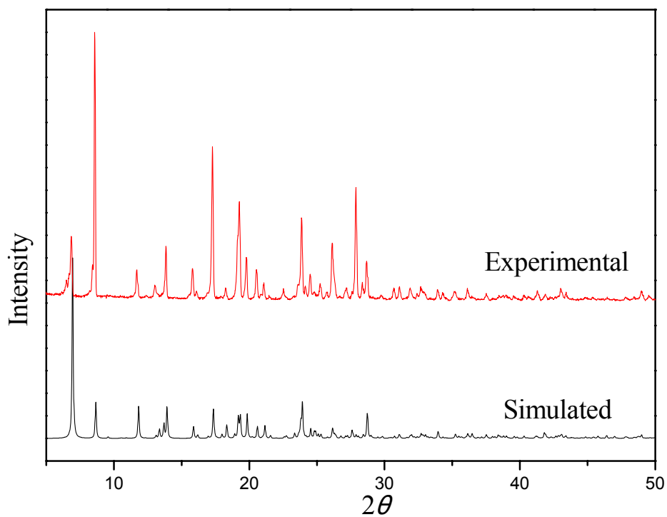
Figure S2. Measured and calculated X-ray powder diffraction (XRD) pattern of 1
