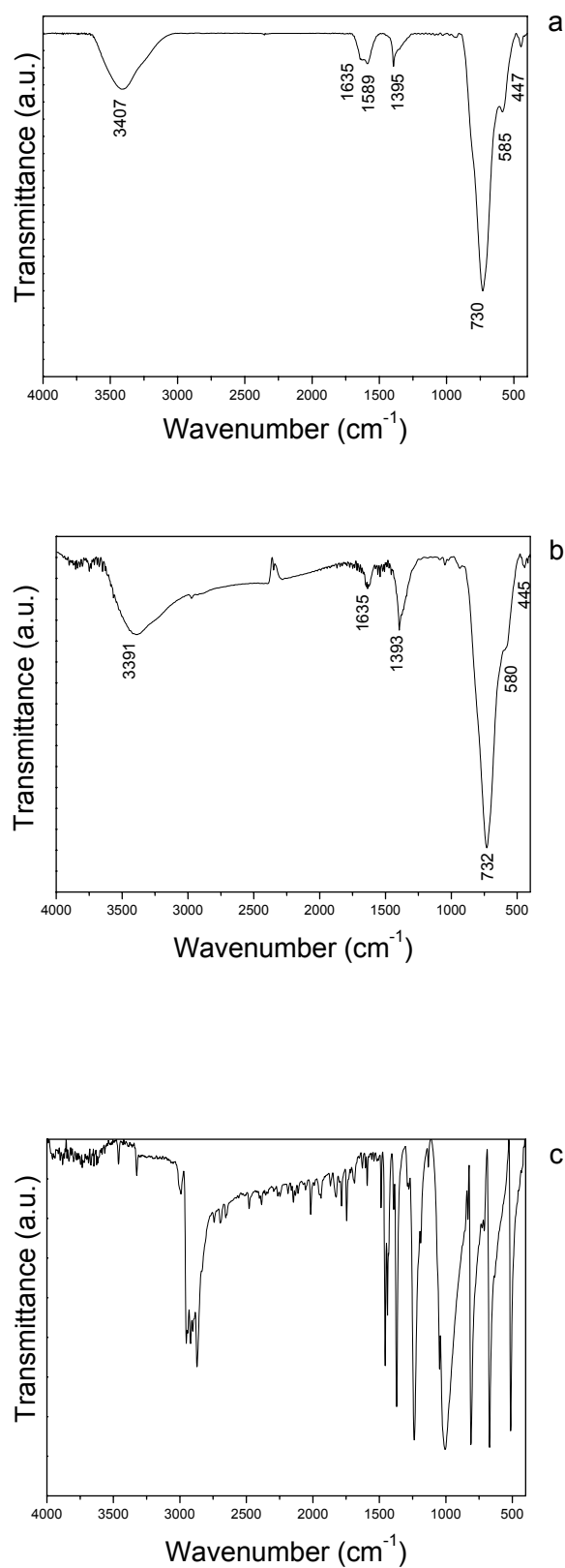
Fig. S1. FT-IR spectra of the products: (a) prepared in the typical experiment; (b) prepared in the absence of HMT; (c) commercial HMT.
