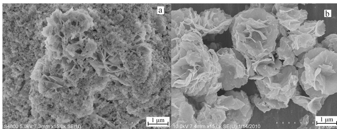
Fig. S2. FE-SEM images of Bi 2 WO 6 obtained at 150 °C after different reaction time: (a) 10 min and (b) 20 min.
