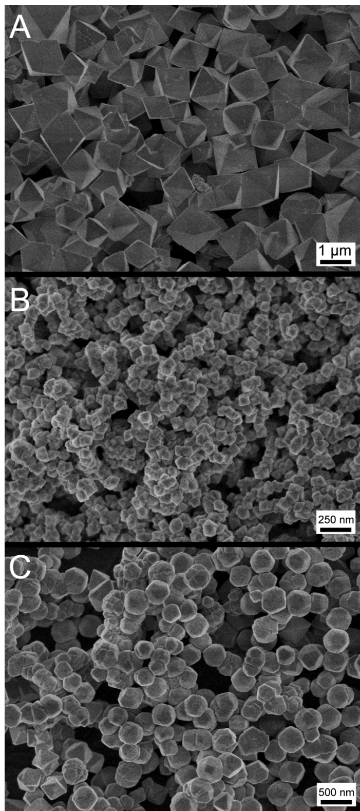
Fig. S2 SEM micrographs of the BiOF 3 (A), BiOF 4 (B), and BiOF 5 (C) samples..
