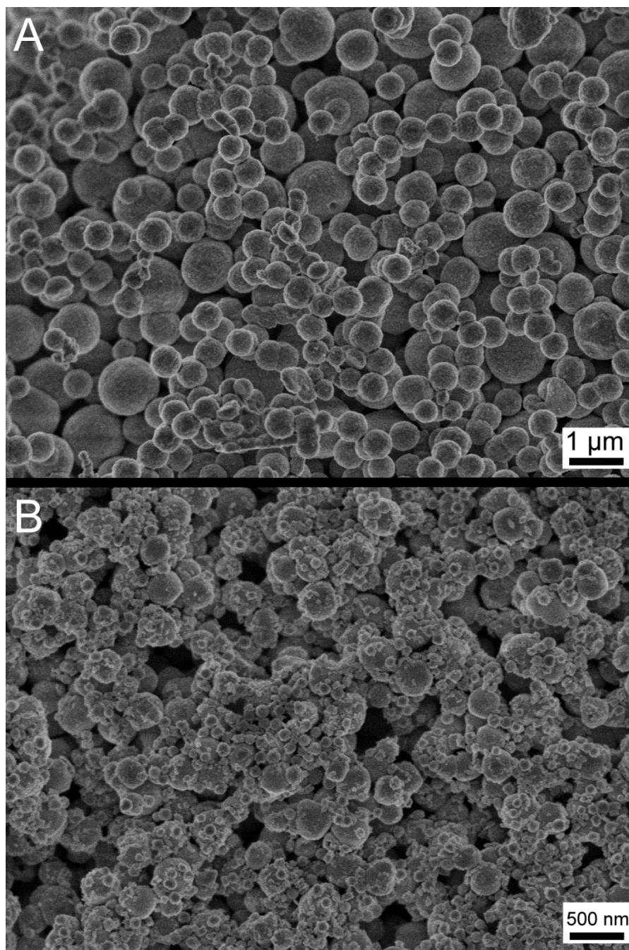
Fig. S3 SEM micrographs of the Bismuth fluoride spheres doped with 5% mol Eu (A) and bismuth oxyfluoride particles doped with 7 % Eu (B).
