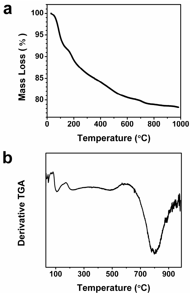
Fig. S1 (a) Thermogravimetric and (b) differential thermogravimetric analyses of powdered tube material obtained under budding conditions.
