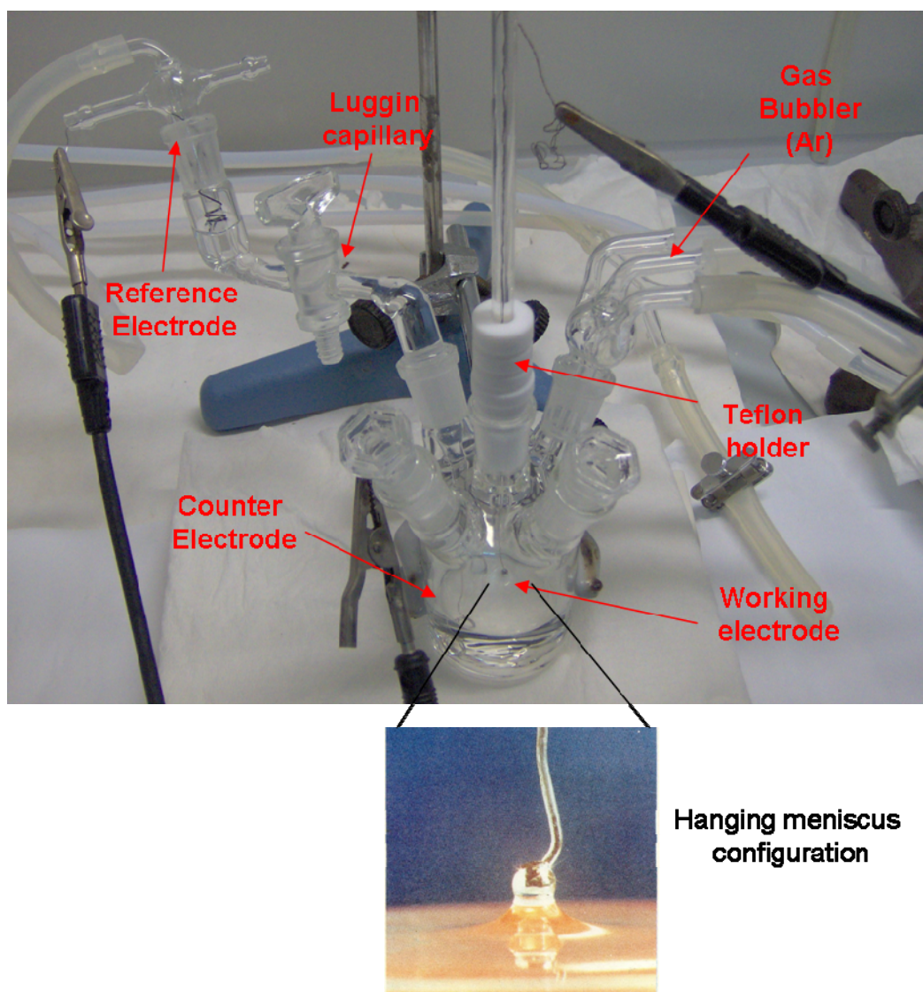
Figure SI1. Picture of the electrochemical cell.
