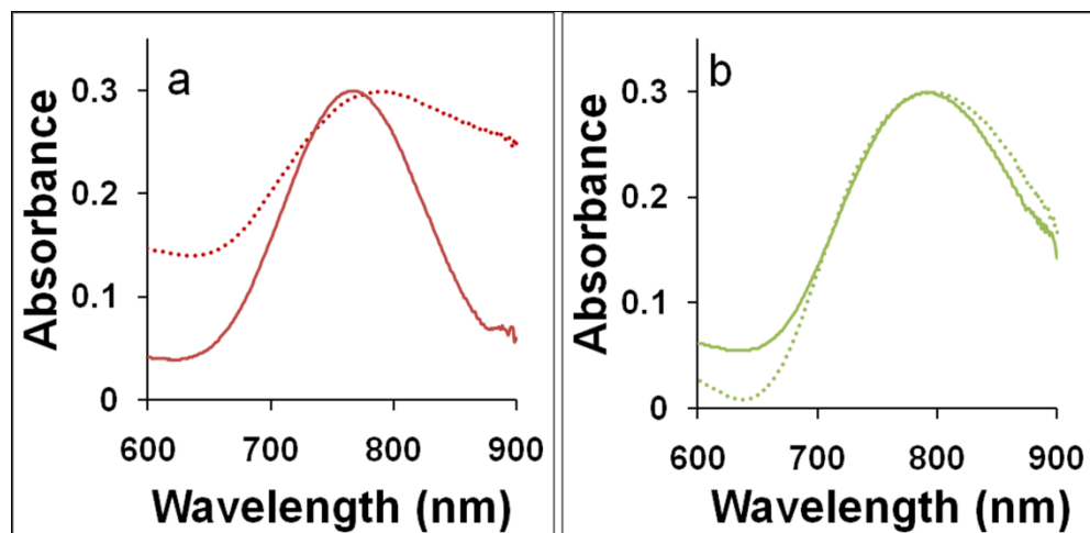
Figure S1: Absorption spectra of GNR@SH-PEG (a) and GNR@SiO 2 @PE-PEG (b) in aqueous solution (solid line) and in cells (dashed lines). The spectrum of GNR@SH-PEG inside cells is broadened and red-shifted by ~20 nm, whereas that of GNR@SiO 2 @PE-PEG shows negligible changes before and after cell uptake.
