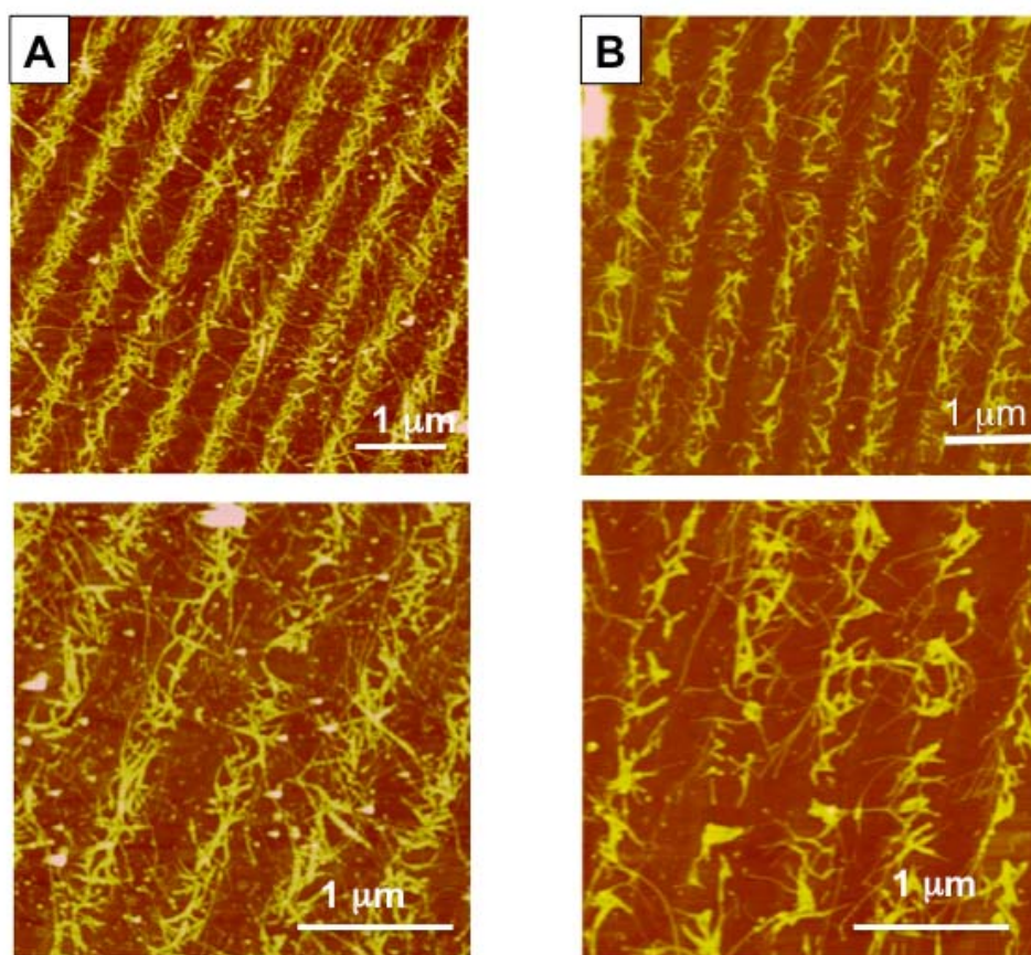
Supplementary Figure 1. (A) AFM images of T 30 -(TC) 7 dispersed CNTs adsorbed on printed (AG) 7 lines from buffers containing 100mM NaCl (top: 5 µm x 5 µm. bottom: 3 µm x 3 µm) (B) AFM images of T 40 -(TC) 7 dispersed CNTs adsorbed on printed (AG) 7 lines from buffers containing 100mM NaCl. top: 5 µm x 5 µm. bottom: 3 µm x 3 µm)
