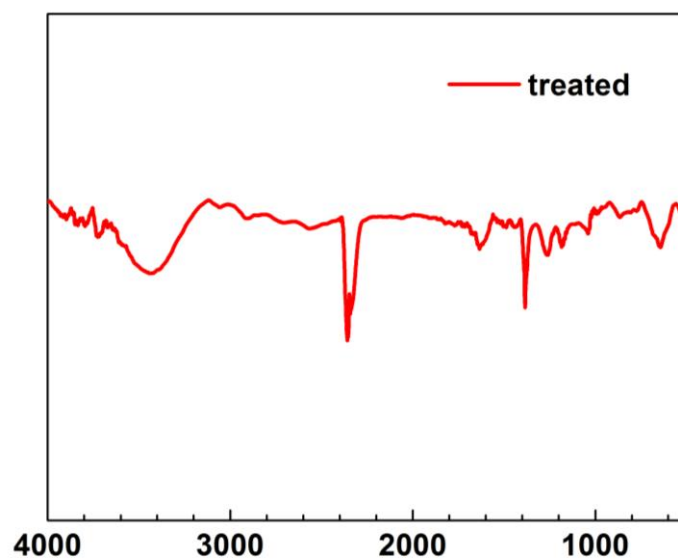
Figure S1. FTIR spectra of the treated carbon paper after soaking in the electrolyte for 2 h.
