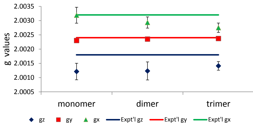
Figure S7. The principal values of the g-tensors of positive, P^+ , polarons on PCDTBT model oligomers (methyl substituent, see above) averaged overall all conformers (standard deviation shown as error bars) as a function of oligomer length. B3LYP functional; def2-TZVPP basis set for ^{32}\text{S} , EPRII basis set for ^{14}\text{N} , ^{12}\text{C} and ^1\text{H} . Further details of the calculations are provided in the Experimental Procedures. These values are generally insensitive to oligomer length and, with the exception of g_y , slightly underestimate the experimental values.
