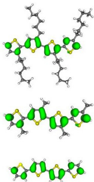
Figure S2. Spin density isosurface plot (contour level of 0.002 \text{ e/a}_0^3 ) for the P3HT tetramer (trans conformer) with complete hexyl sidechains ( top ), for the methyl substituted tetramer ( middle ), and the hydrogen substituted tetramer ( bottom ). B3LYP functional; def2-TZVPP basis set for ^{32}\text{S} , EPRII basis set for ^{12}\text{C} and ^1\text{H} . The spin density does not extend to the alkyl chain and is similar for all three molecules.
