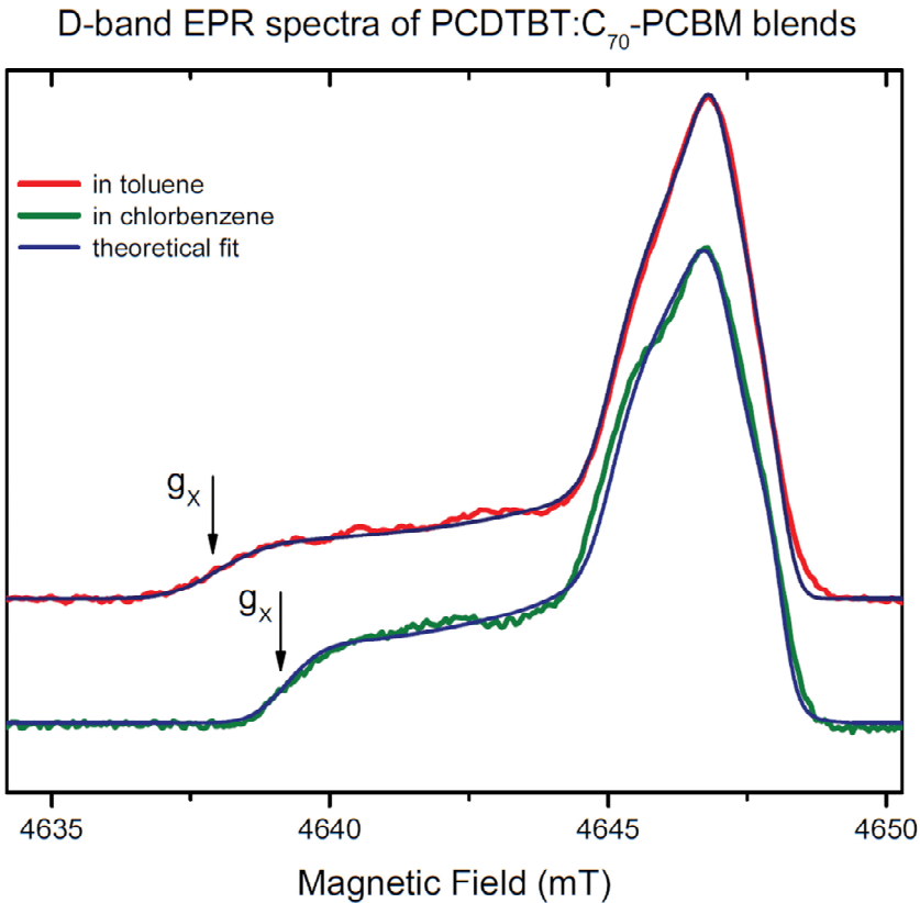
Figure S11. Echo-detected D-band EPR spectra of PCDTBT: C_{70} -PCBM blends using toluene (Red) or chlorobenzene (Green) as solvent. Illuminated at 50 K. Simulations of the experimental spectra are shown in Blue. The low field component of C_{70} -PCBM ^- , g_x , exhibits a large g-strain effect, which reveals in the large linewidth of this component and indicates the sensitivity on its direct surrounding. Slight variations of g_x value, in the order of \pm 0.0002 , were observed in different samples prepared in toluene solution. The use of chlorobenzene instead of toluene as solvent also had a slightly larger effect on this g-value. Table S6 provides the principal g-values of C_{70} -PCBM anions used for the simulation.
