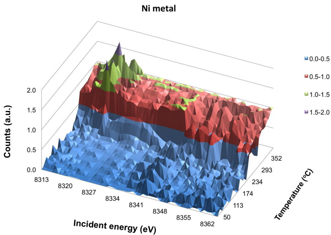
Figure S2: Evolution of Ni 0 contribution to XES signal as a function of reduction temperature and incident beam energy.
