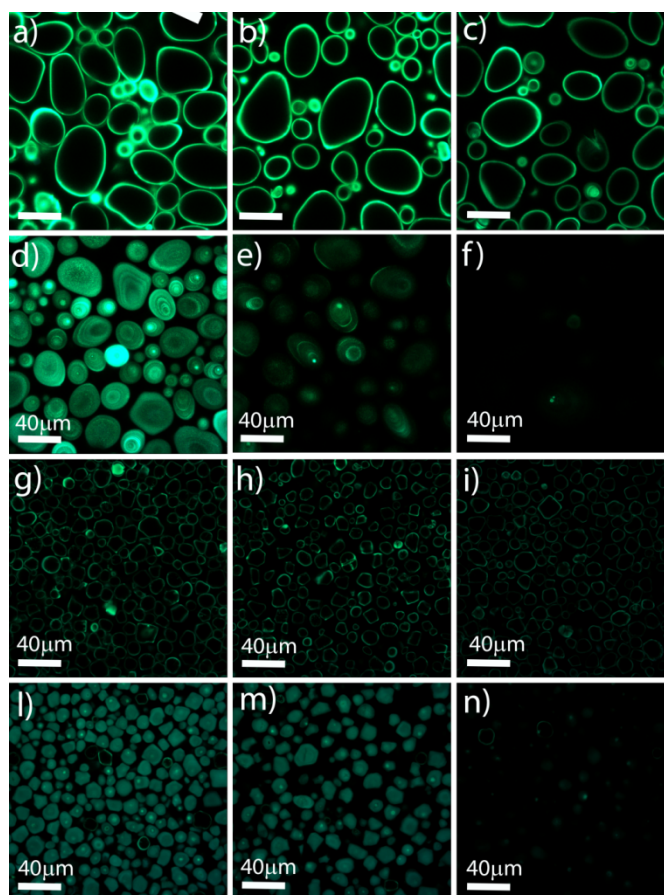
Fig. S1: CLSM images of regular potato (a), waxy potato (d), regular corn (g) and waxy corn (l) starch granules in suspension 7 days after the addition of 5-hexadecanoylamino fluorescein molecules. The images b, e, h, m refer to the same starch species acquired after the “washing” procedure with 50% DMF. The images c, f, i, n refer to the same starch species acquired after the “washing” procedure with 90% DMF.
