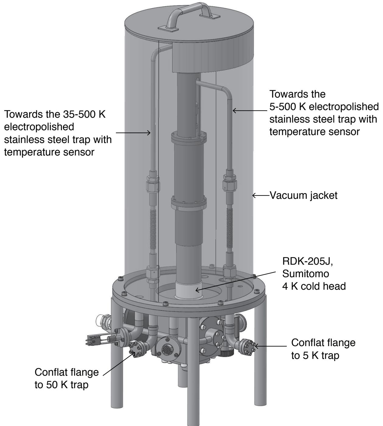
Figure S1. Schematic of the dual stainless steel cryogenic trap fabricated by Janis Research Company, complementary to Figure 1. The design is considered proprietary by Janis Research, therefore the full schematic is not shown.
