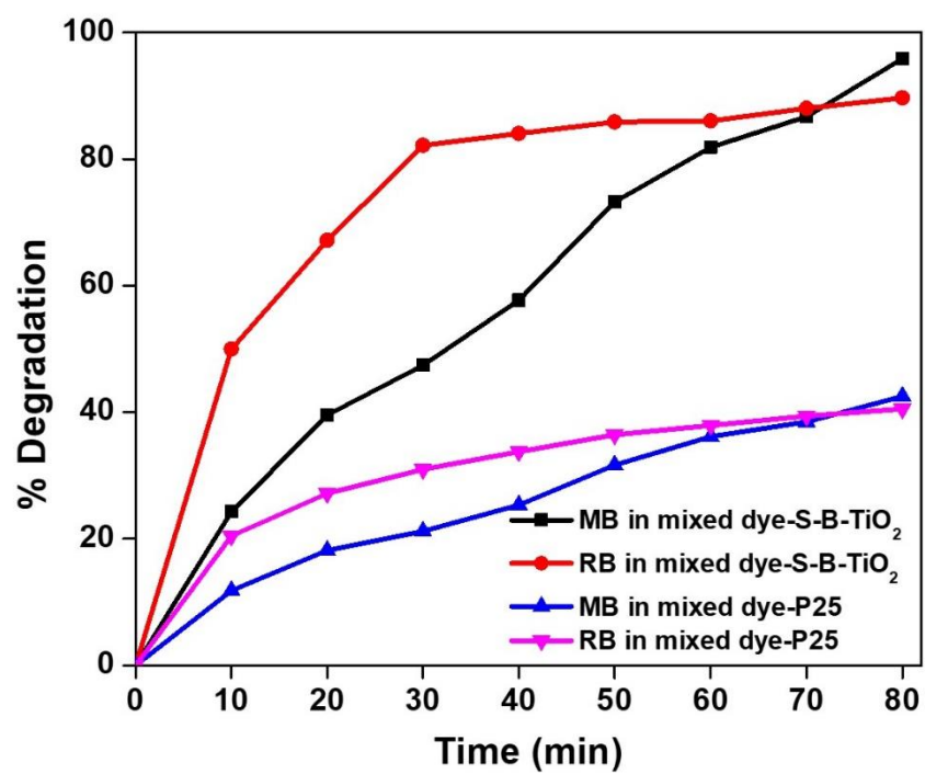
Figure S2: Comparative degradation studies of S-B-TiO 2 and P25.
