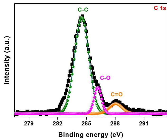
Figure S1: XPS spectrum of carbon.
