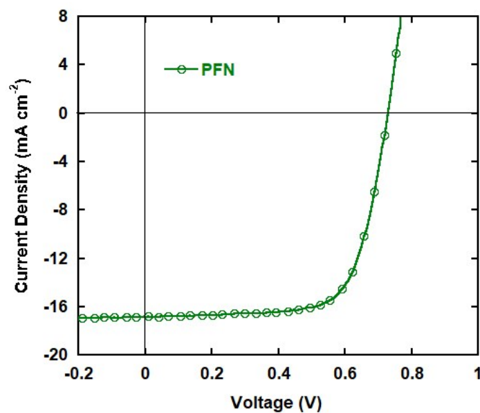
Figure S3. J - V curve of inverted PTB7:PC 71 BM PSC with PFN CBL.
