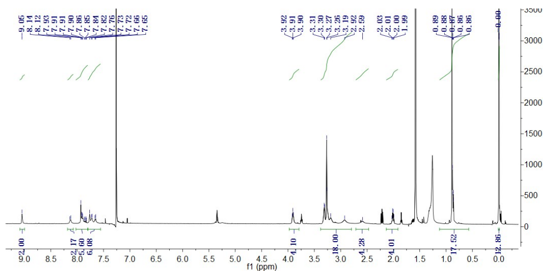
Figure S1. 1 H NMR of PFSOPy-E in CDCl 3 .
