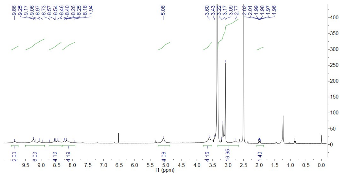
Figure S2. ^1\text{H} NMR of PFSOPyCl-E in \text{DMSO-d}_6 .
