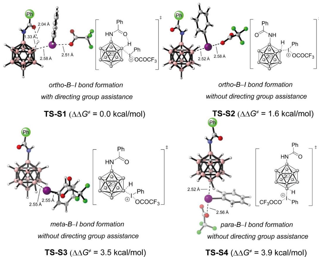
Fig. S1. Relative free energies and optimized structures of competing B–I bond formation transition states with trifluoroacetate leaving group.
