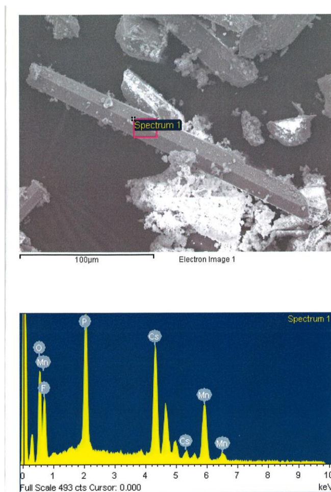
Figure 1. SEM image (top) and EDX spectrum (bottom) for \text{Cs}_2\text{Mn(III)}_2\text{F}_4(\text{PO}_3\text{F})_2 (compound VII)
