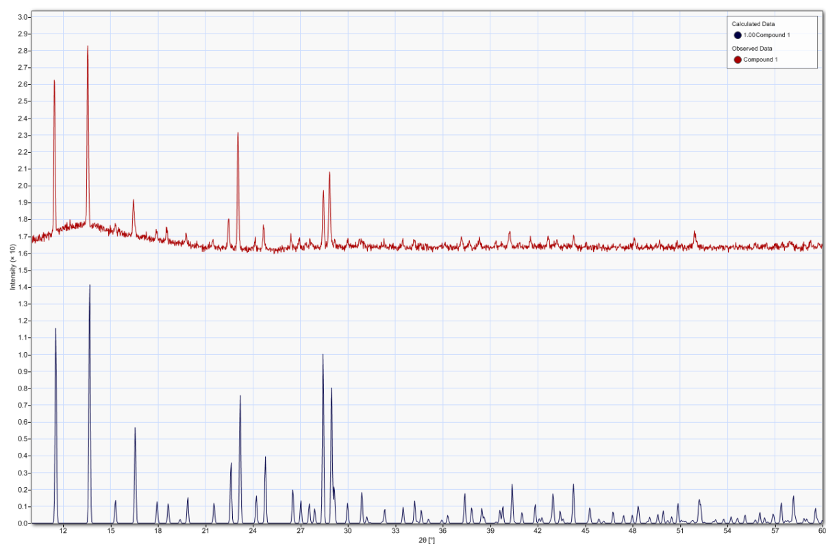
Figure S1. Calculated (blue) and experimental (red) PXD pattern for compound I
