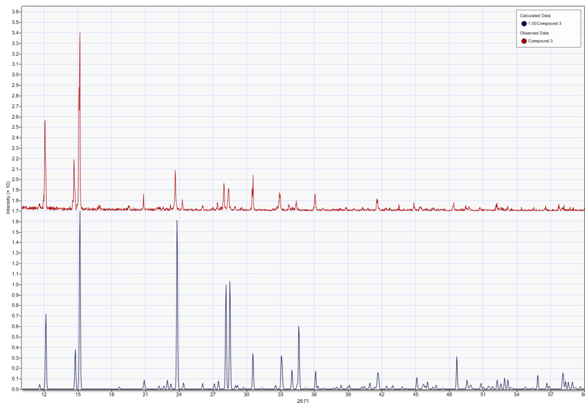
Figure S2. Calculated (blue) and experimental (red) PXD pattern for compound III
