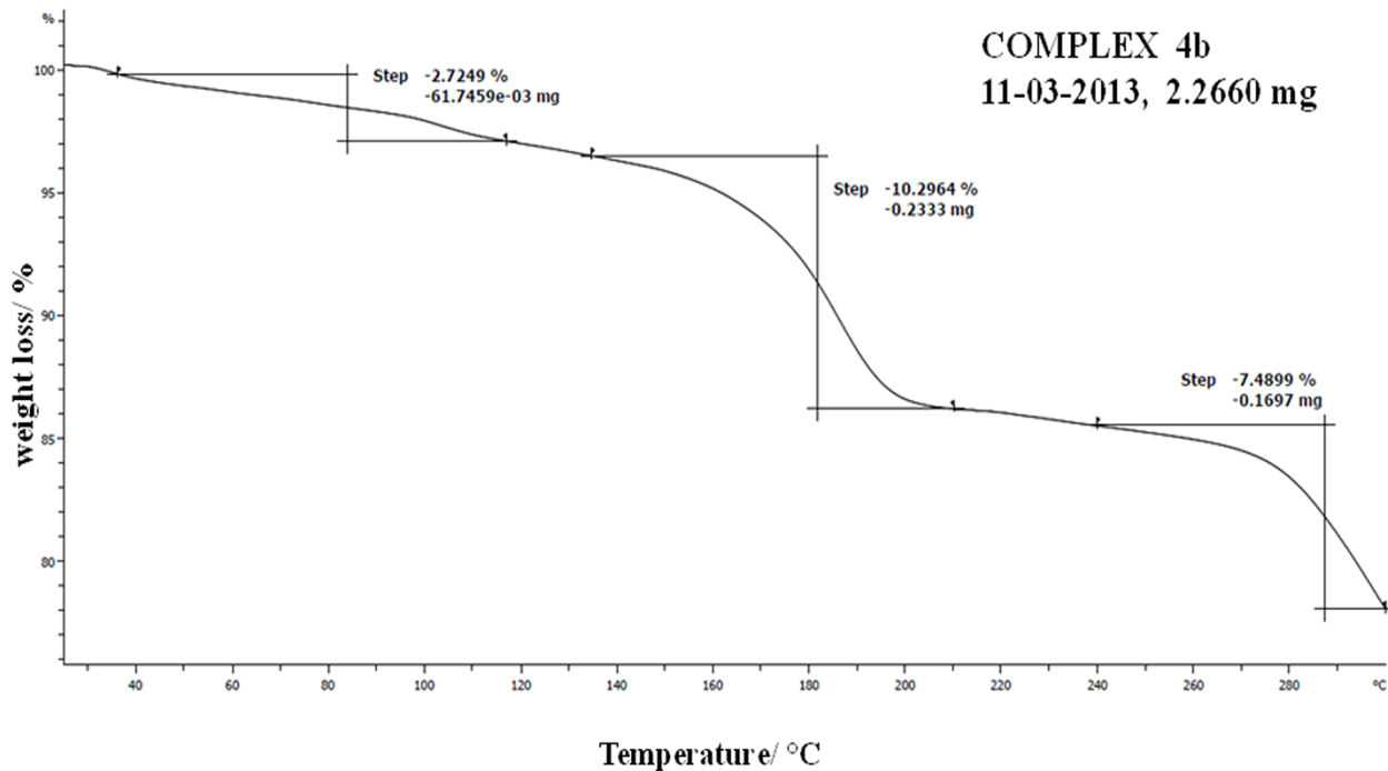
Figure 3 Thermogravimetric curve of compound 4b . Plot of weight loss/ % against temperature/ °C.
