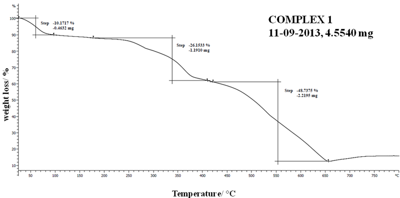
Figure 1 Thermogravimetric curve of compound 1 . Plot of weight loss/ % against temperature/ °C.
