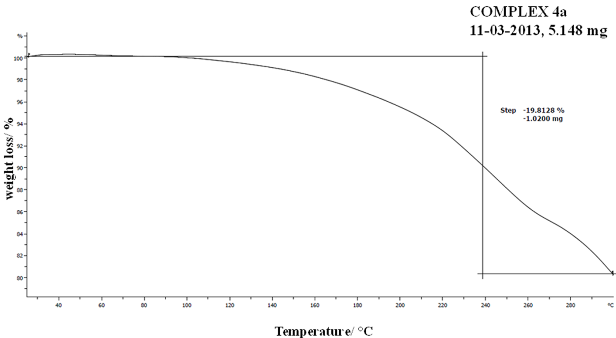
Figure 2 Thermogravimetric curve of compound 4a . Plot of weight loss/ % against temperature/ °C.
