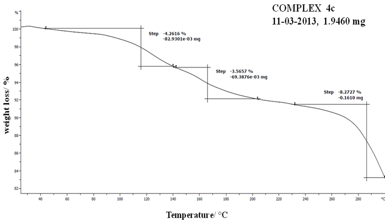
Figure 4 Thermogravimetric curve of compound 4c . Plot of weight loss/ % against temperature/ °C.
