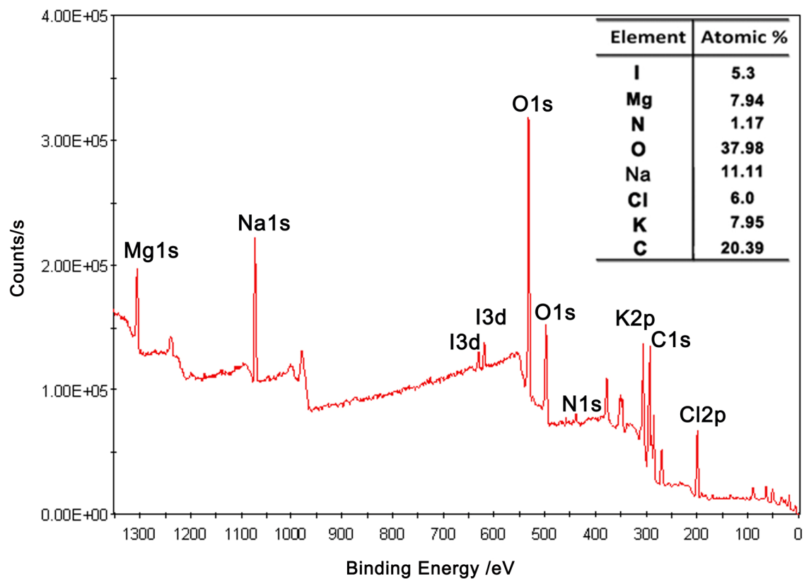
Figure S1. XPS pattern in all elements binding energy region of kelp , with the inset of atomic contents of each element.
