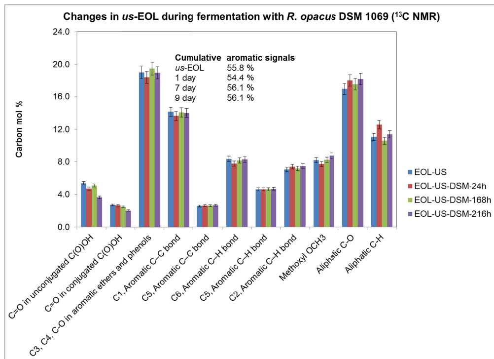
Figure S2 Results from ^{13}\text{C} NMR experiments obtained on microbially modified us -EOL samples
