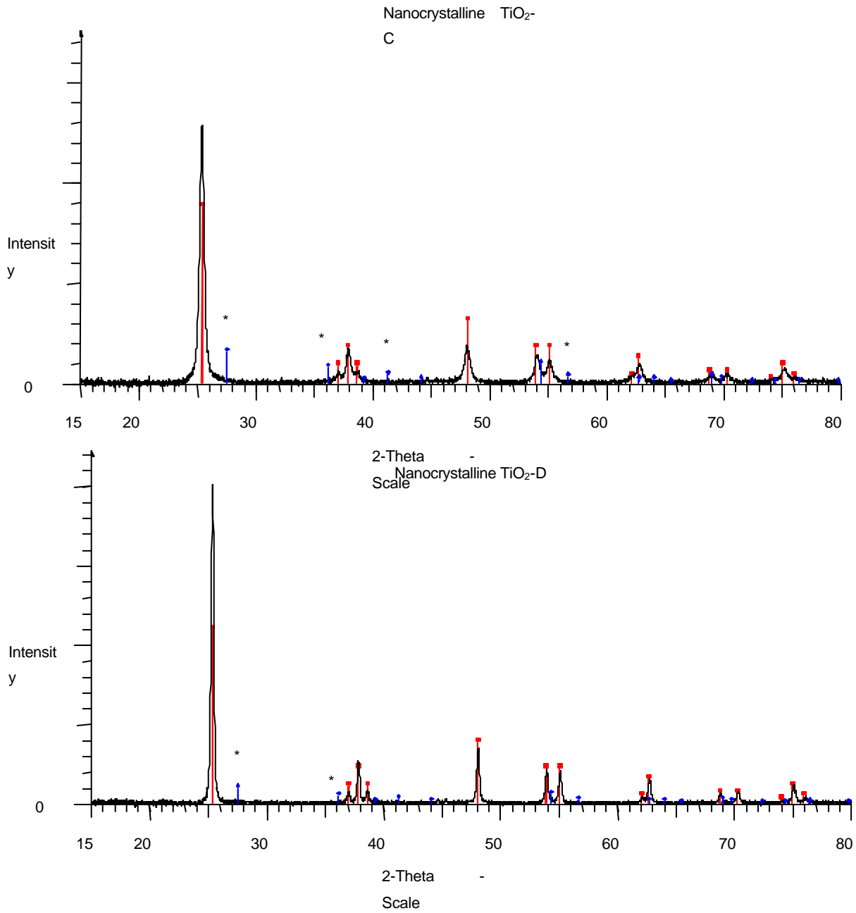
Figure 1. XRD data for of Nanocrystalline TiO 2 . Rutile phases are indicated in Blue. Almost no formation of the rutile phase is observed.
