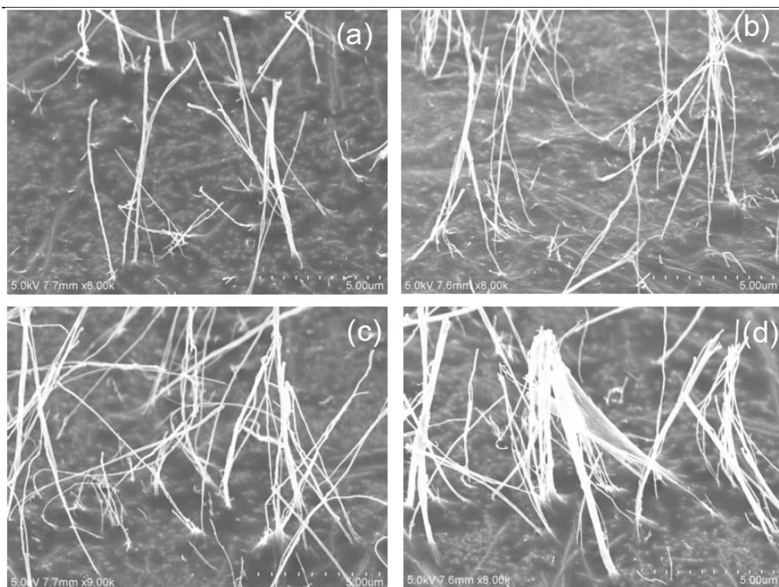
Fig. S2. SEM images of CNTs transferred on Scotch tape with different pre-press force (a, 4; b, 8; c, 16; d, 32 N cm -2 ). All scale bars: 5 μm.
