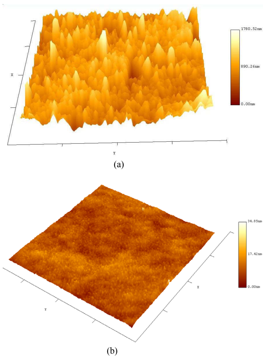
Fig. S1. Surface AFM images of vertically aligned CNTs (a) and adhesive layer of a Scotch tape (b). Scale: 10 \times 10 \mu\text{m} .
