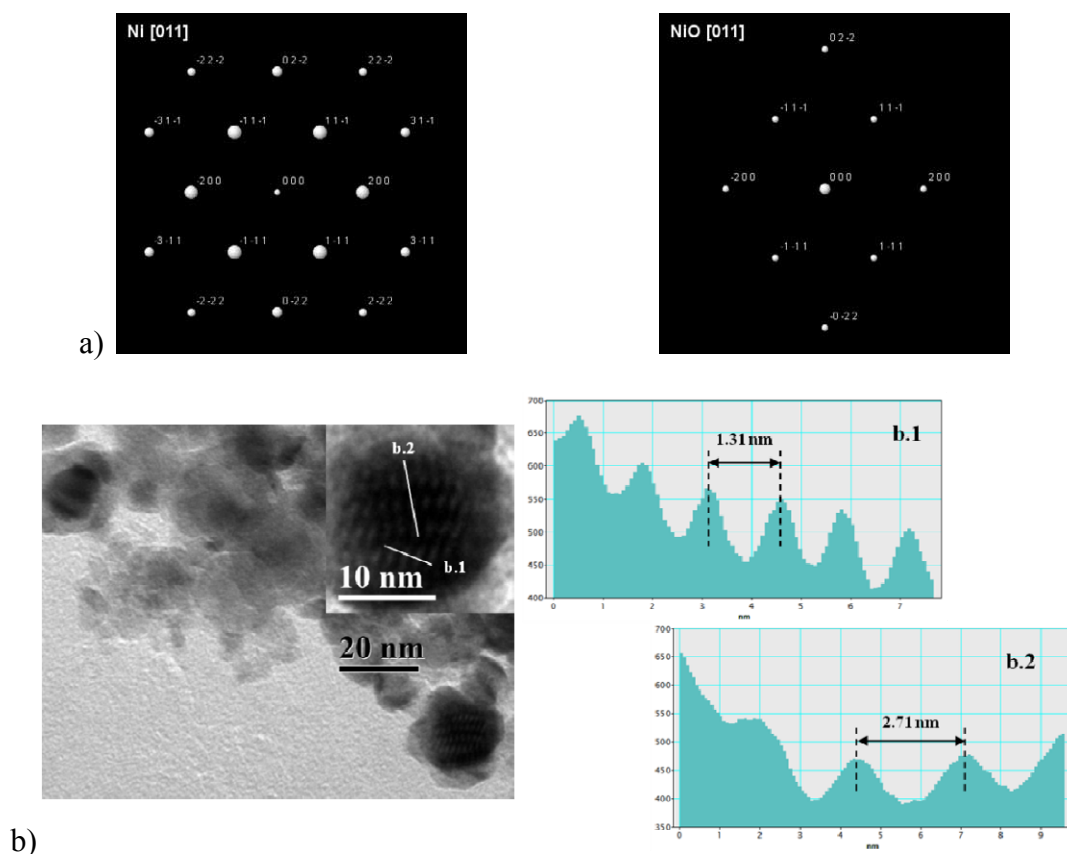
Figure S3. (a) Expected diffraction patterns for Ni (left) and NiO (right) under the [011] zone axis; (b) TEM image of sample No. 3. The spacings of the moiré fringes are indicated in the intensity profiles at the right, which have been obtained from linear sections (b.1 and b.2) normal to the orientation of each set of fringes (white lines in the inset).
