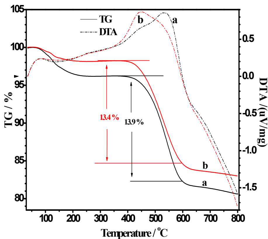
Fig. S1 DTA-TG curves of (a) HZSM-34-S and (b) HZSM-34-HT samples.
