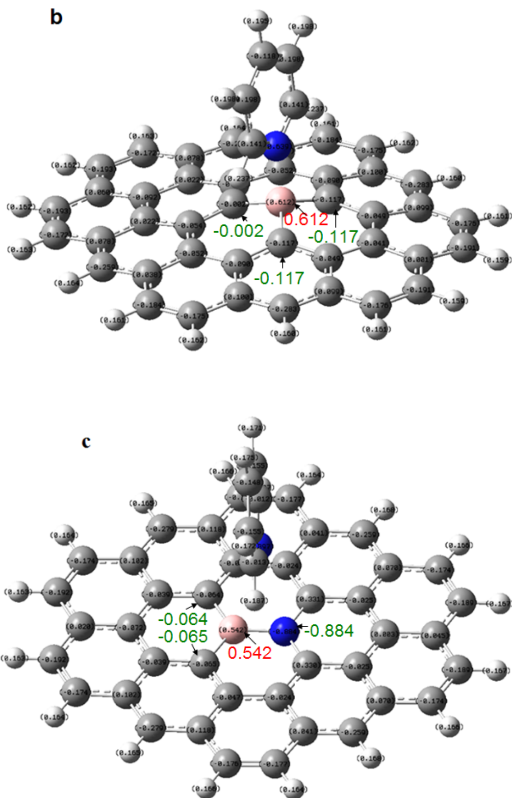
Figure S1. The calculated mulliken charge distributions of (a) pyridine-mono vacancy graphene, (b) pyridine-B substituted graphene, (c) pyridine-BN substituted graphene.
