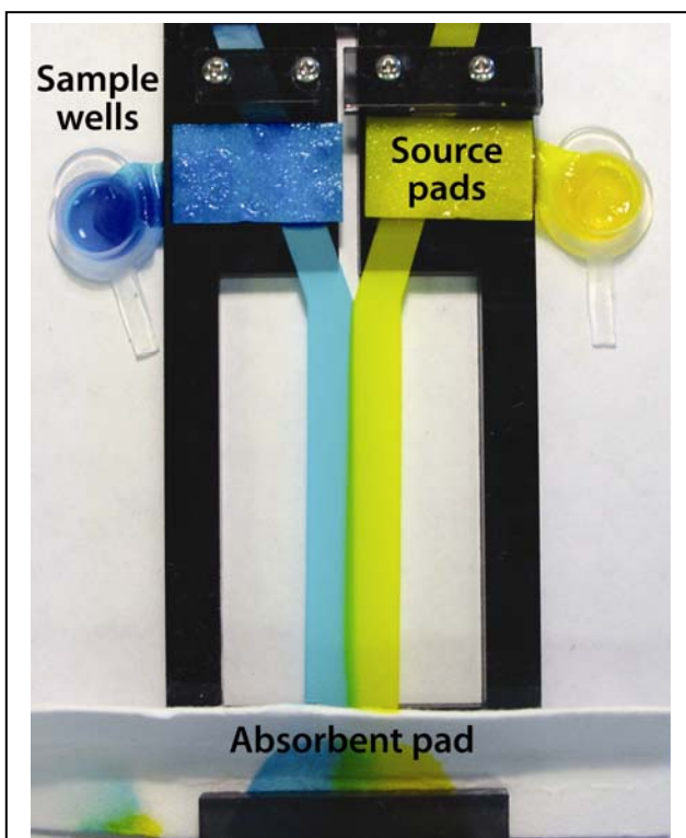
Fig S1. An image of a fully assembled 2DPN showing the sample wells, PMMA jig, source pads and absorbent pad.
