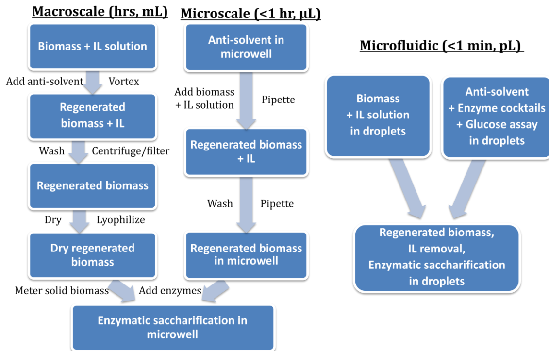
Figure S1: Workflow for determination of sugar released from biomass using conventional, microscale and microfluidic approaches.
