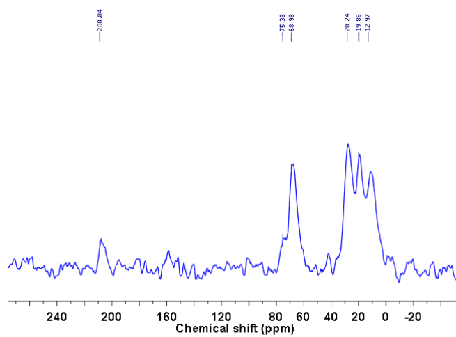
^{13}\text{C} CP-MAS NMR spectrum of M-(acac) 5 .
