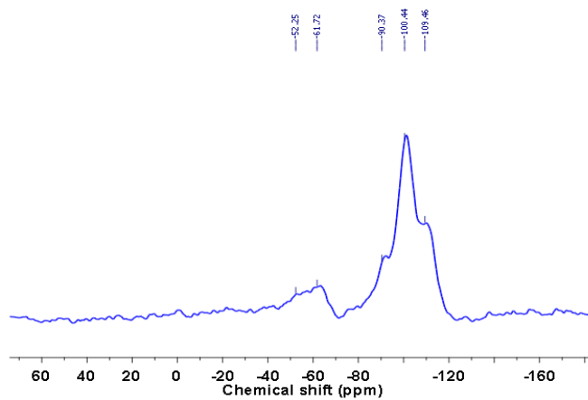
^{29}\text{Si} CP-MAS NMR spectrum of M-(acac) 5 .
