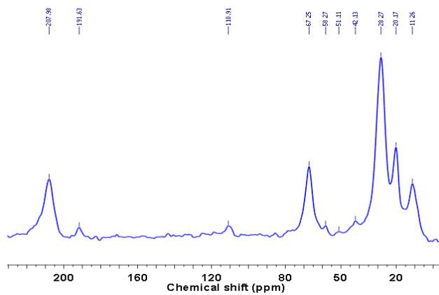
^{13}\text{C} CP-MAS NMR spectrum of M-(acac) 10 .
