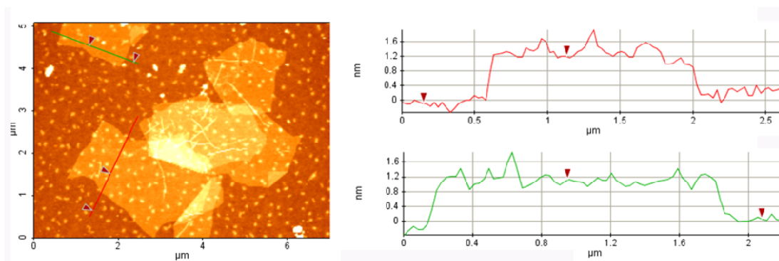
Fig. S1: AFM image of single-sheet graphene oxide. The small dot-like features are inorganic salt particles on the surfaces of SiO 2 /Si substrates.
